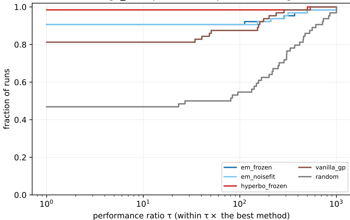
shrinkage_a0.3: performance profile (final regret)
