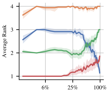
RMSE
