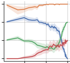
CRPS
