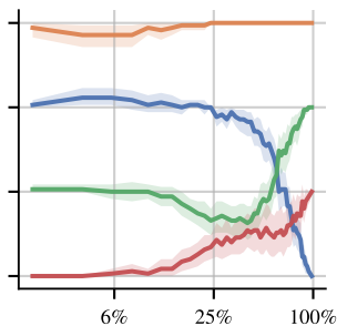
CRPS
