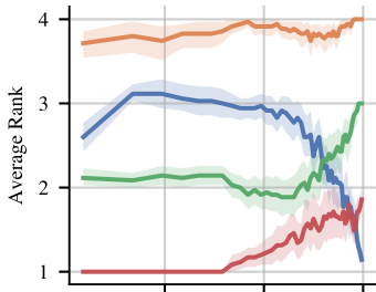
RMSE
