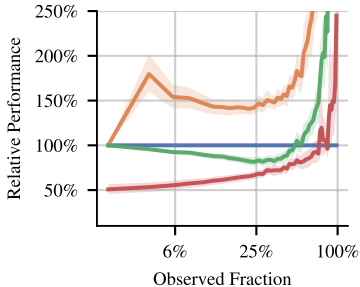
RMSE
