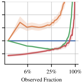
CRPS
