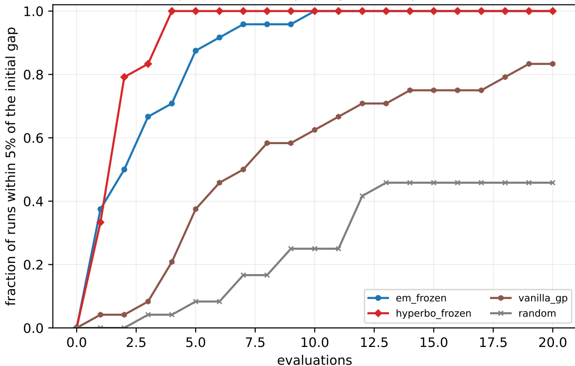
Batch BO q=4, MC-fantasy qLogEI: data profile (tol=5%)
