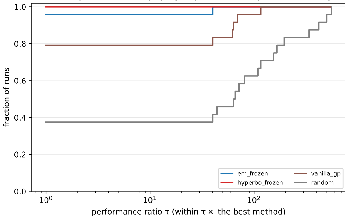
Batch BO q=4 , MC-fantasy q\text{LogEI} : performance profile (final regret)
