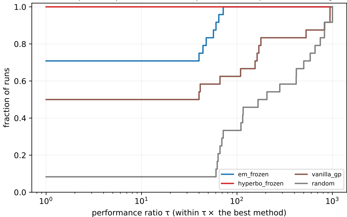
Batch BO q=1 (sequential control): performance profile (final regret)
