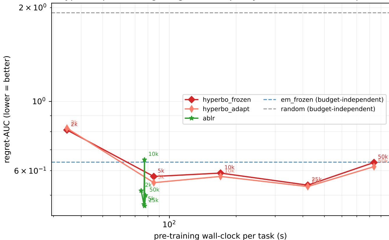
HyperBO pre-training budget vs BO quality (LCBench, 192 runs/point)
