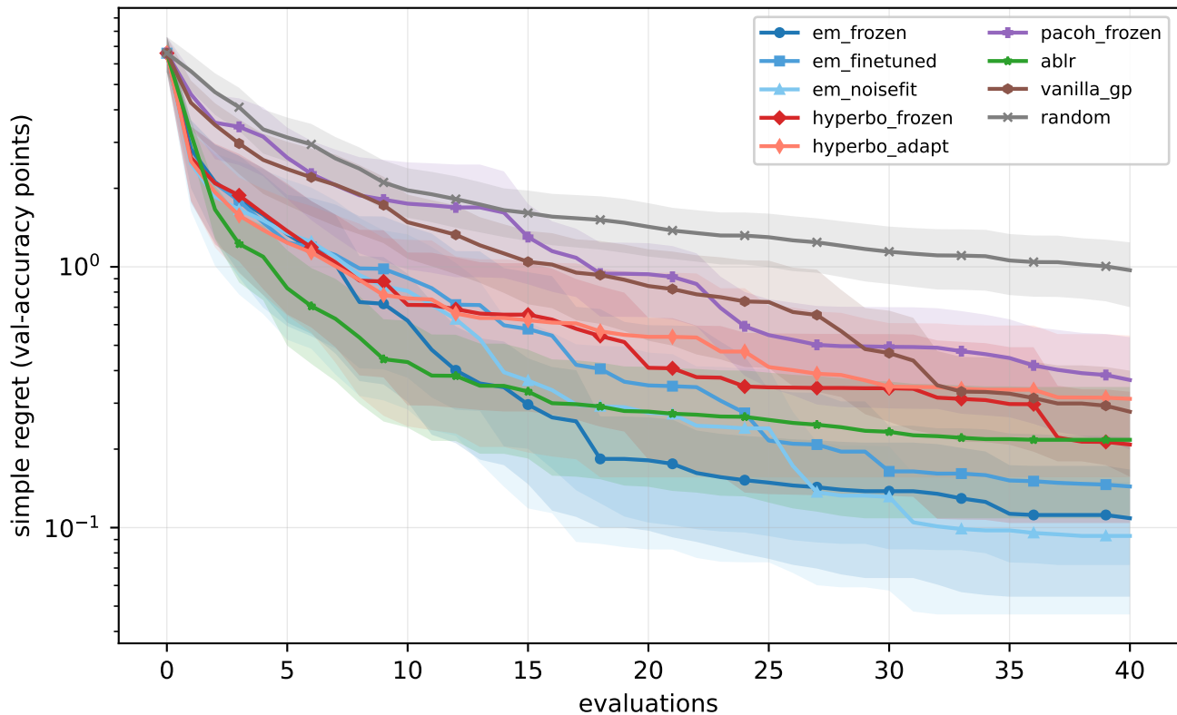
LCBench 7D BO (12 datasets x 16 seeds)
