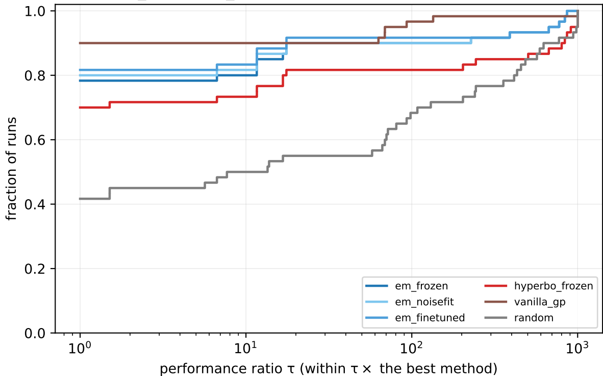
ood_shrinkage_a0.3: performance profile (final regret)
