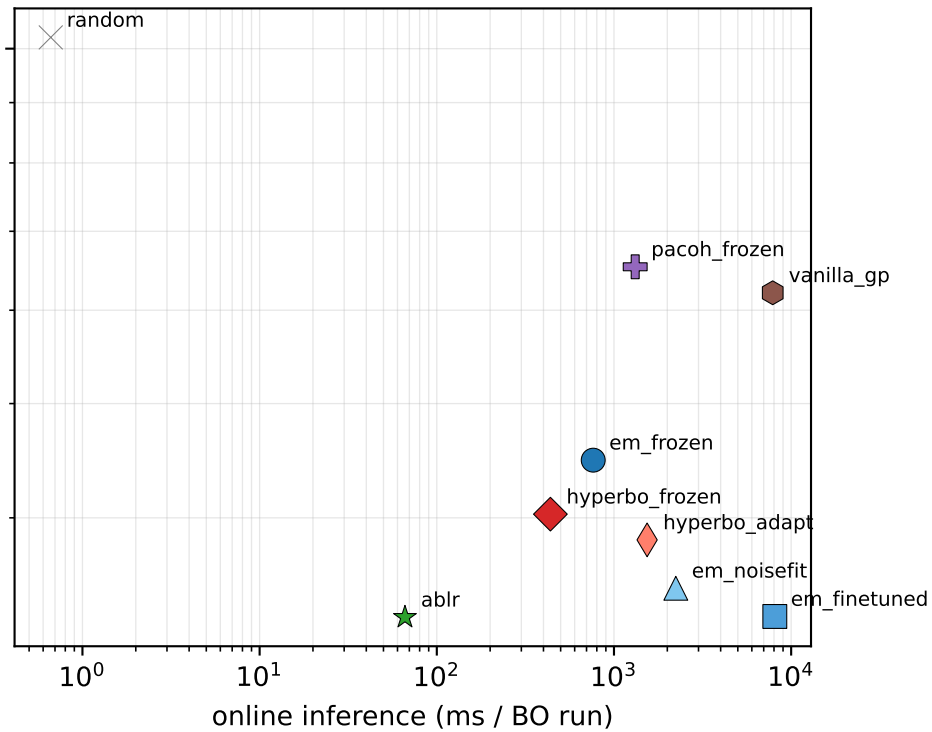
PD1 full: LOO over 23 tasks, neglog warp (115 runs) - quality vs cost (bottom-left is best)
