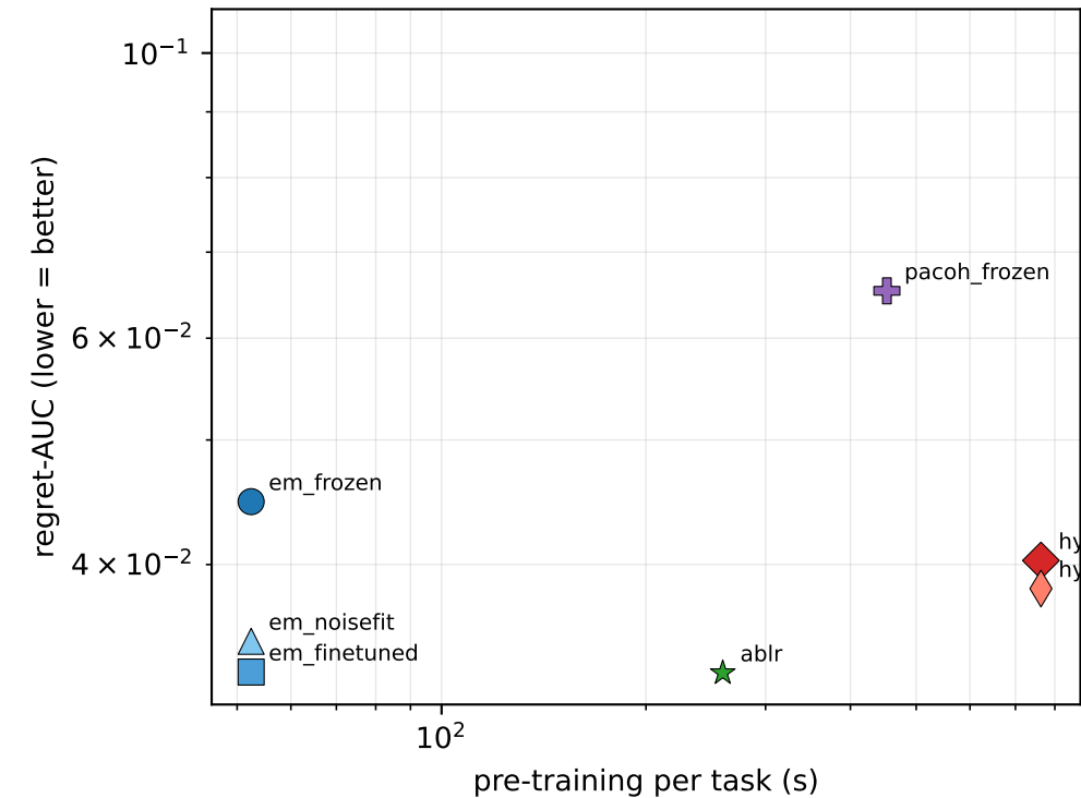
PD1 full: LOO over 23 tasks, neglog warp (115 runs) - quality vs cost (bottom-left is best)
