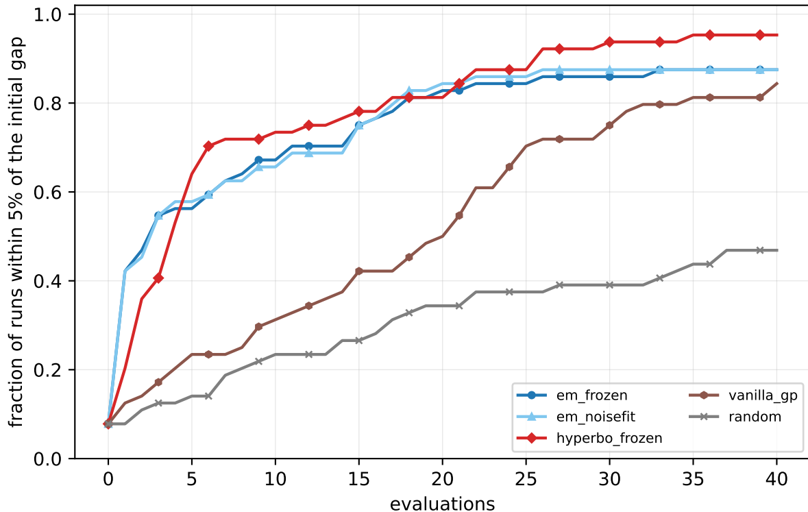
shrinkage_a0.3: data profile (tol=5%)
