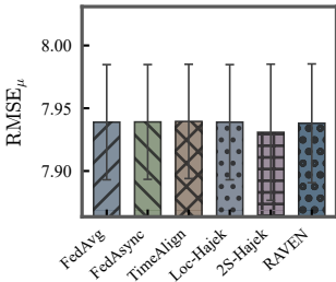
(a) SensorScope, RMSE_{\mu}
