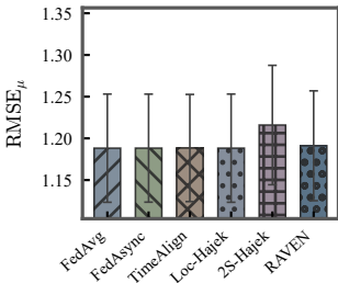
(c) U-Air, RMSE_{\mu}
