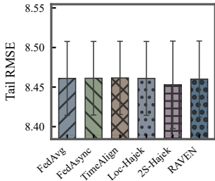
(b) SensorScope, Tail RMSE
