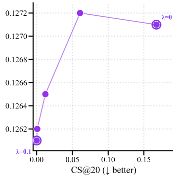
PACER-Full
