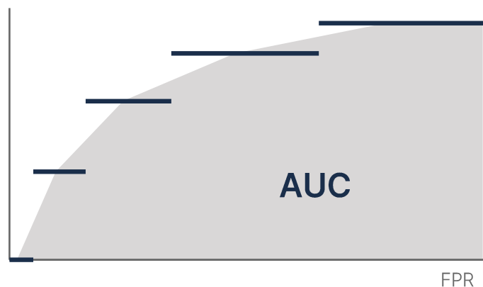
ROC Curve
