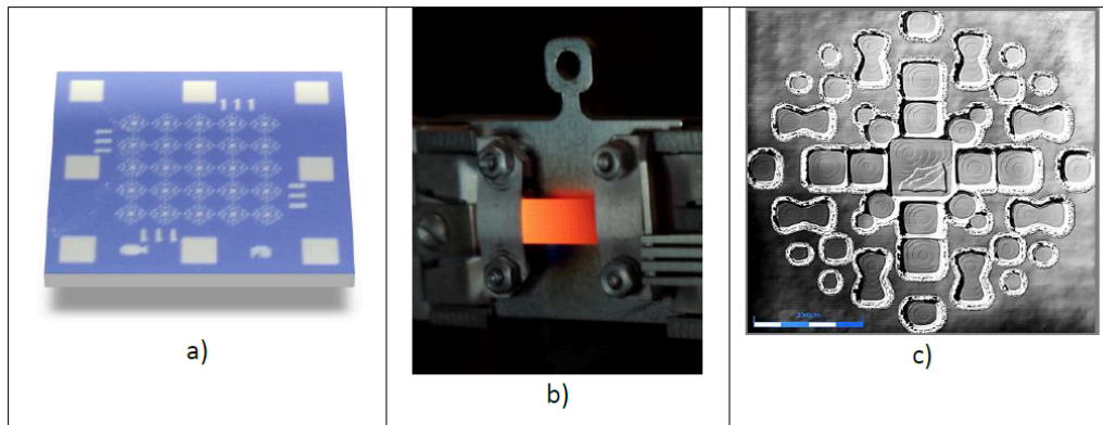
Figure 6 — Steps showing the Si samples preparation. a) after oxidation and e-beam lithography with 5 \times 5 fields, b) during annealing at high temperature in UHV, c) image on one field obtained by LSCM.
