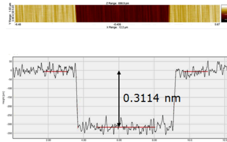
Figure 8 — Amphitheatre-like arrangement of steps and use of an evaluation in analogy to ISO 5436 to determine the step height (from J. Garnaes, DFM)
