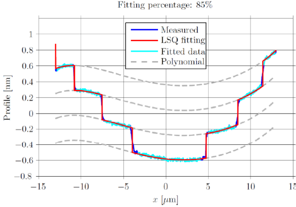
Figure 9 — Use of a polynomial fit to correct for scanner deviations by J. Garneas [to be published]. Here a polynomial of fourth order was sufficient. Result of 4th order: d_{\text{cor}} = (0.3137 \pm 0.0038) nm, that is, u(d_{\text{cor}}) = 1.2\% .
