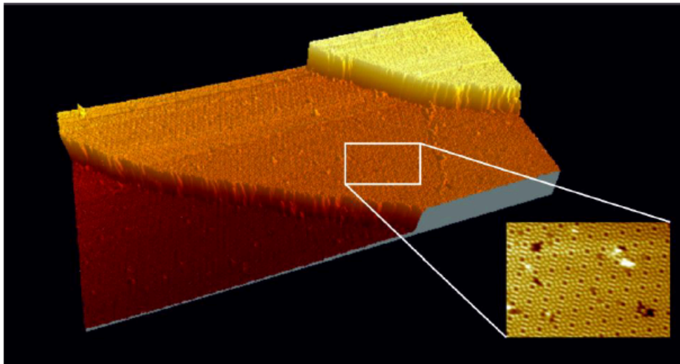
Figure 3 — Atomically resolved Si(111) - 7 \times 7 surface showing two monoatomic steps in UHV.
