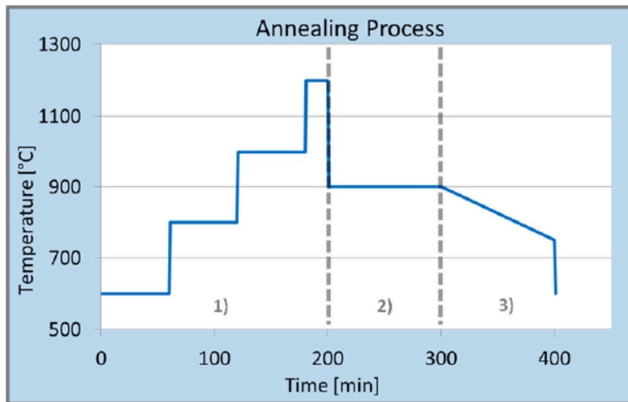
Figure 7 — Schematic of the temperature profile for annealing Si samples. The first temperature ramp is a further cleaning step in which the sample is cleaned of remaining foreign atoms (1). While holding the sample at approx. 900^\circ\text{C} (section 2), the Si surface lattice is reconstructed into a 7 \times 7 structure. In the course of the last temperature ramp, the terraces or atomically smooth areas are formed by self-organization (3).
