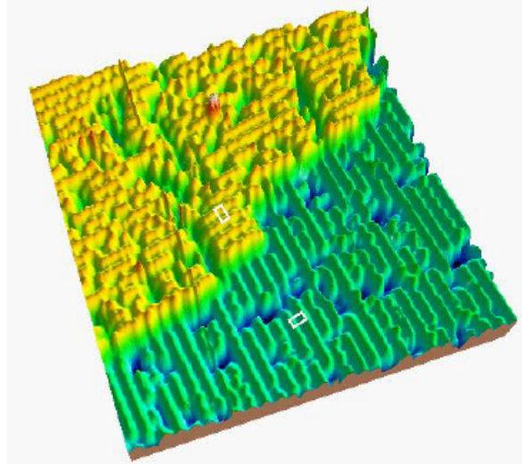
Figure 2 — Si(100) 2 \times 1 surface with a monoatomic step of 0.13 nm. Two unit cells indicated on the lower and one on the upper plane rotated by 90^\circ .
