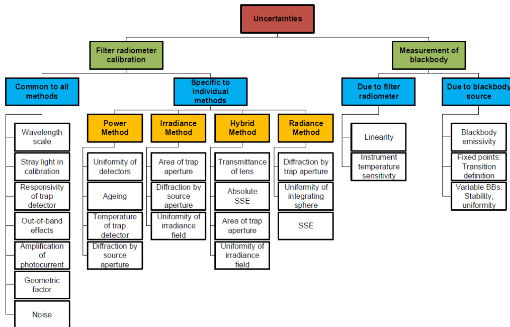
Figure 5 — Classification of the uncertainty components.
