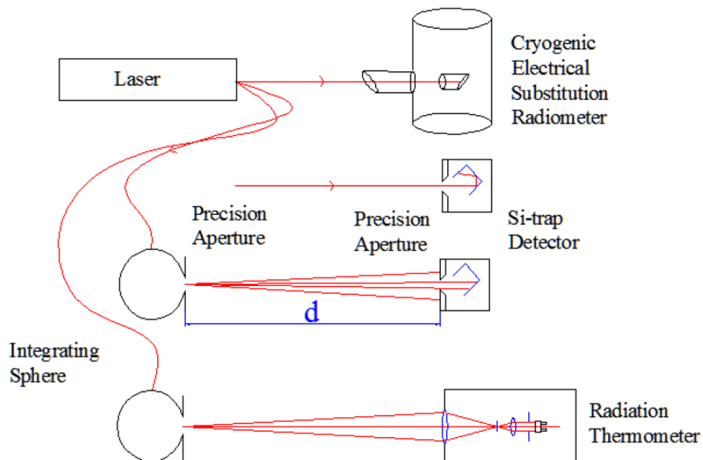
Figure 4 — The radiance method.
