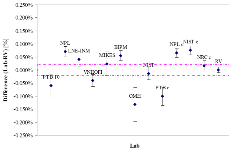
Figure 6 — Comparison result for aperture area (from CCPR-S2 report).
