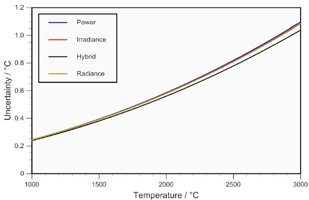
Figure 14 — Uncertainties for each calibration scheme, propagated from the normal values given in Table 10 and Table 11.
