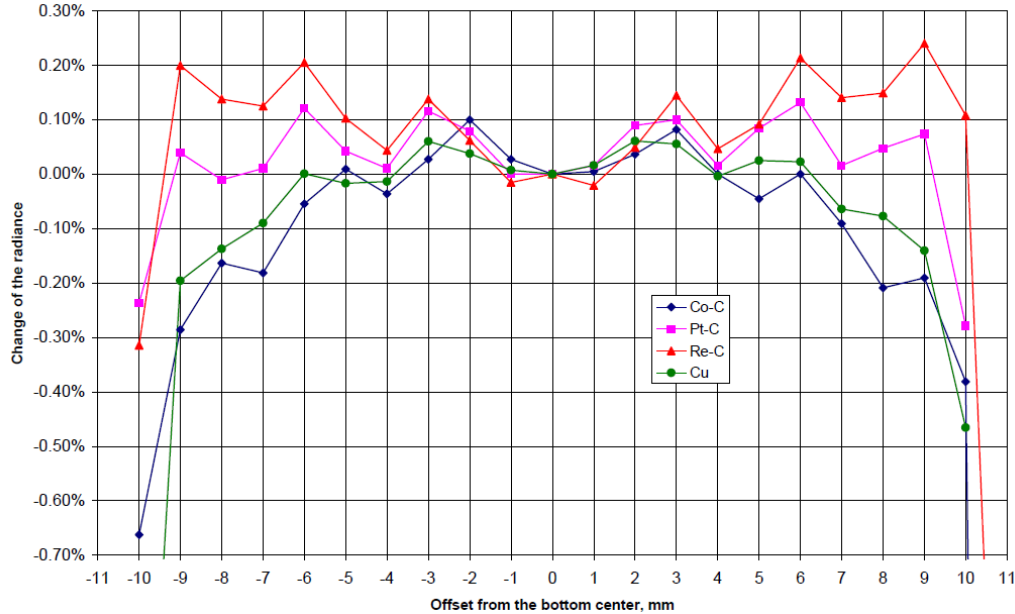
Figure 13 — Cavity bottom uniformity of the blackbody BB3500M measured at VNIIOFI for Co-C, Pt-C, Re-C, and Cu points. The measurements were carried out at a wavelength of 900 nm for the Cu point, and 650 nm for the other three points.
