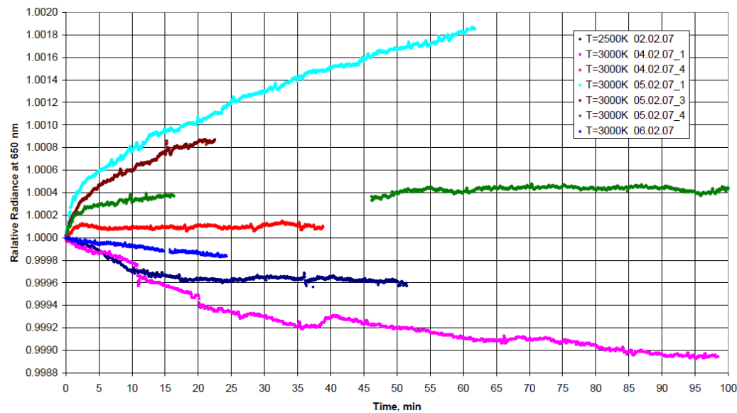
Figure 12 — Typical stability of the actively stabilised VTBB of the BB3500 type.
