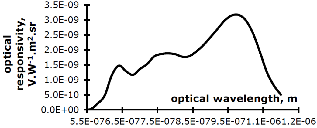
Figure 9 — Optical responsivity of a spectroradiometer.
