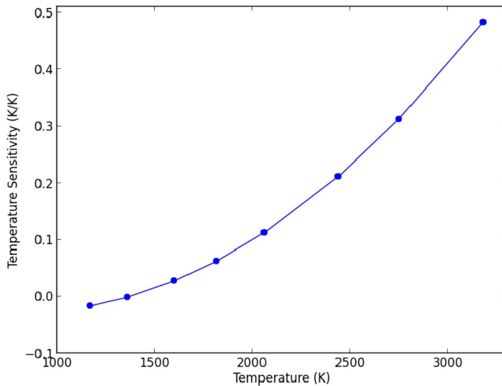
Figure 11 — Change in the measured temperature (of a blackbody, for example) indicated by 650 nm, glass filter-based FR per degree of FR operating temperature change.
