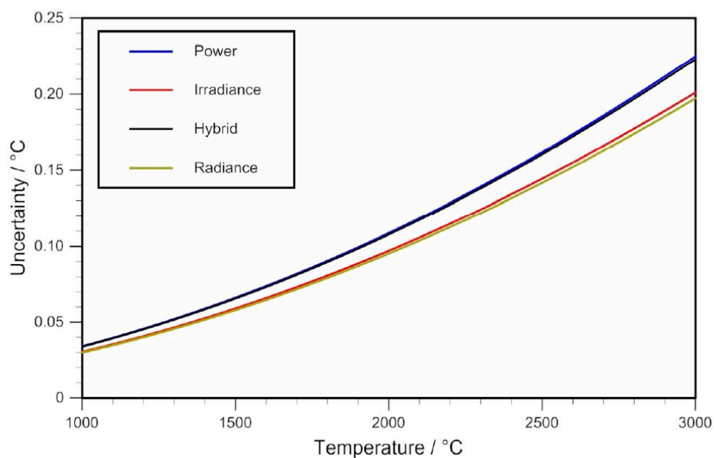
Figure 15 — Uncertainties for each calibration scheme, propagated from the best values given in Table 10 and Table 11.
