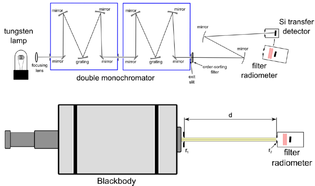
Figure 8 — Calibration and use setups for the power method.
