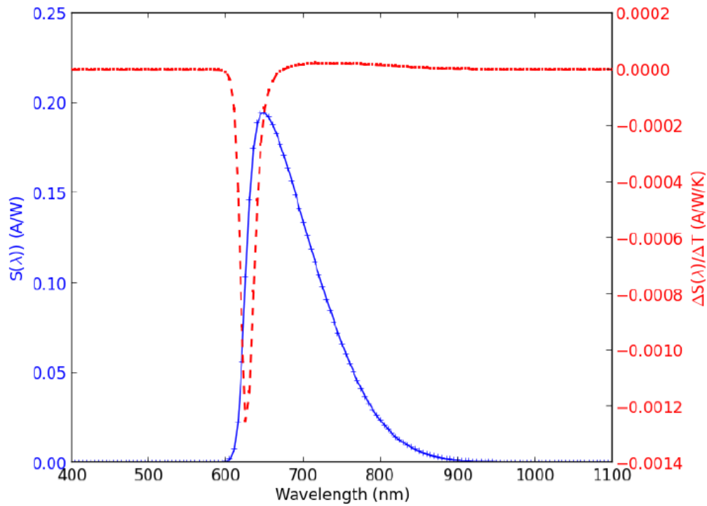
Figure 10 — Responsivity (blue) and the change in responsivity with temperature (red) for a glass filter, Si detector filter radiometer with a central wavelength near 650 nm.
