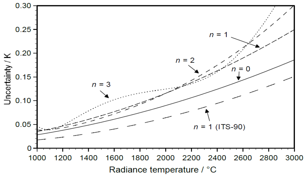
Figure 1 — Comparison of combined standard uncertainties for each of the examples considered above. The curve labelled n = 1 gives the uncertainty in thermodynamic T extrapolated from the gold point assuming an uncertainty in the gold-point temperature as determined by absolute primary radiometry. For n = 1 (ITS-90) the thermodynamic uncertainty associated with the gold-point temperature is not included. The result for the best possible absolute primary radiometric thermometry ( n = 0 ) is also shown for comparison.
