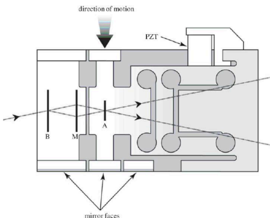
Figure A3.1 — Plan view of a monolithic X-ray interferometer. B, M and A are lamellae.
