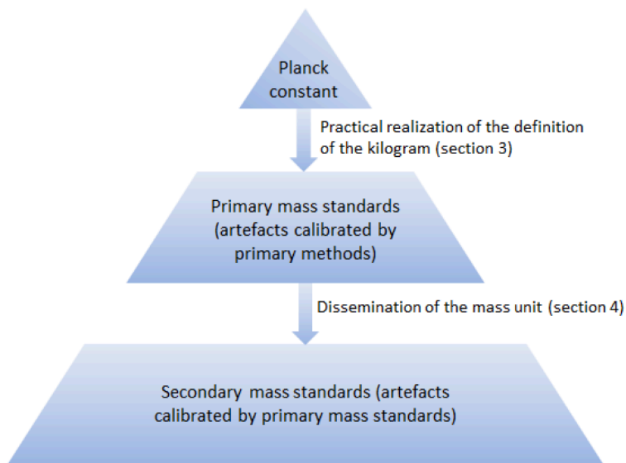
Figure 1 — Illustration of the traceability chain from the definition of the kilogram. The unit of the Planck constant being \text{kg m}^2 \text{s}^{-1} , the units second and metre are needed to derive a primary mass standard from the Planck constant.
