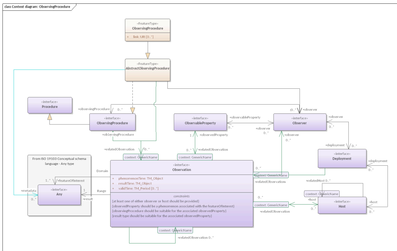
Figure 17 — Context diagram: ObservingProcedure
