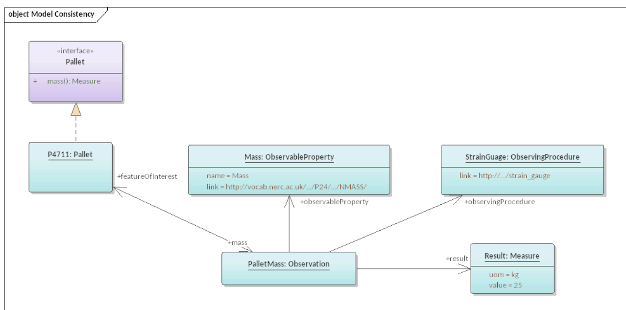
Figure 35 — Model Consistency
