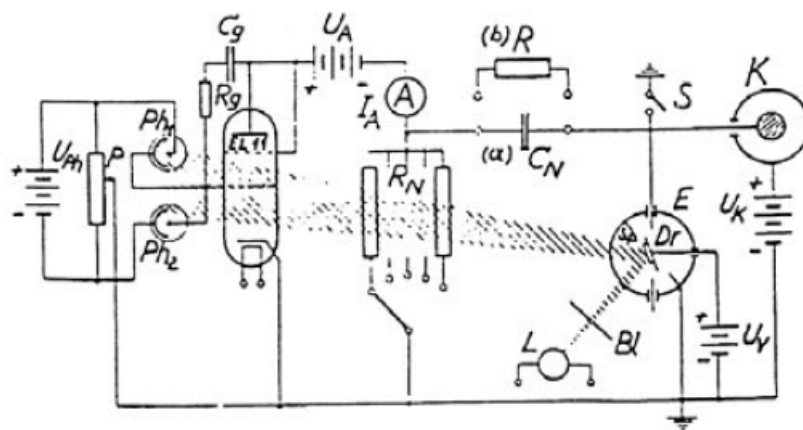
Figure 34 — Electrometer-photocell compensator by Hübner ([222], see p. 178), with ionization chamber K and high tension U_k . The electrometer E with a turning light-mirror system ( L , BI , Dr ) initiates variable currents on the photocells Ph_1 and Ph_2 connected to the vacuum tube EL11 , which itself controls the potential at point (a) by the voltage decrease on the high-ohmic resistor R_N and creating the compensation charge on the collecting capacitor C_N , for zero switch S open. The anode current I_{Ai} of the tube is measured by the instrument A during the time t at the beginning and the end of the compensation giving the ionization current
