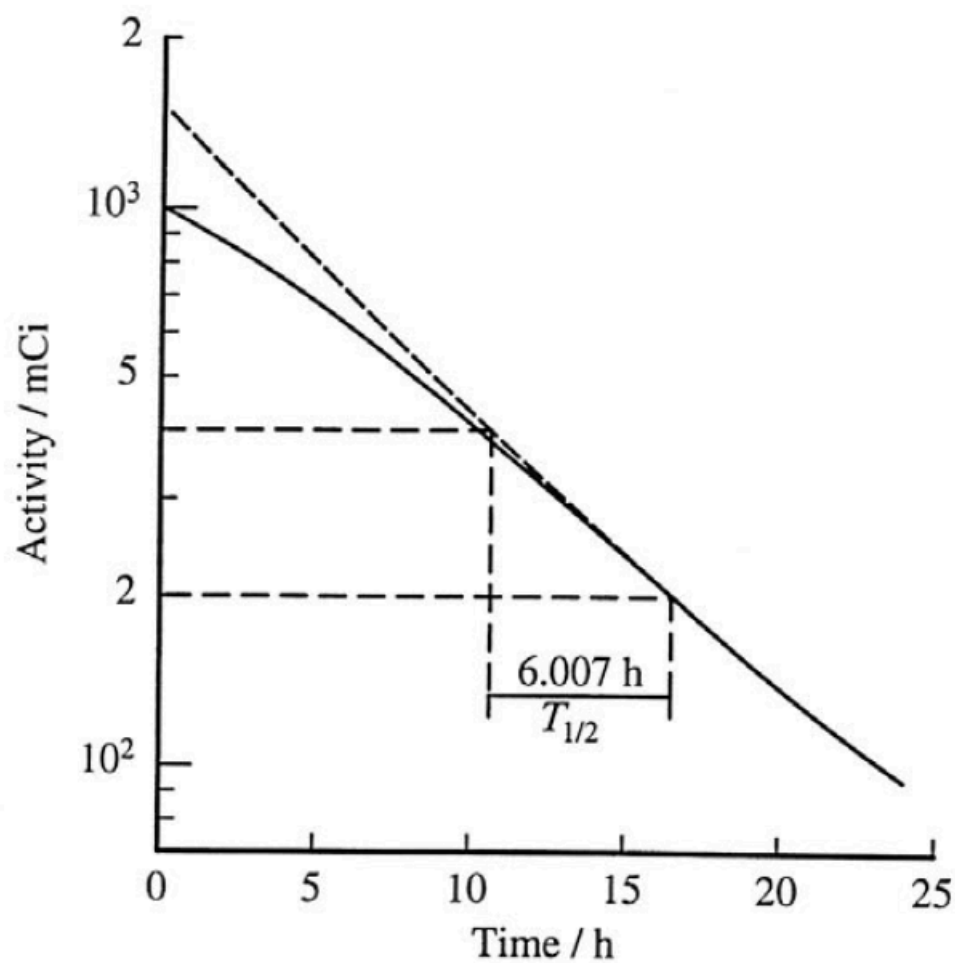
Figure 46-1 — The results for the instrument show smooth deviations from linearity at even low activity values which can only be detected by a half-life analysis for ^{99}\text{Tc}^m .
