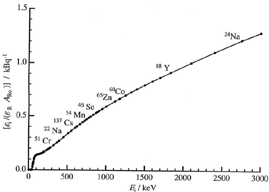
Figure 57 — Photon efficiency \varepsilon versus photon energy E for the PTB ionization chamber, type IG 12 of Centronic (see Figure 14, see p. 94), with various radionuclides. (Unpublished data from PTB).
