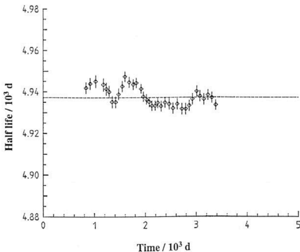
Figure 71-2 — Half-life values are plotted from fits of various data subsets with lower number of data points and shorter time period versus an average time for each subset.
