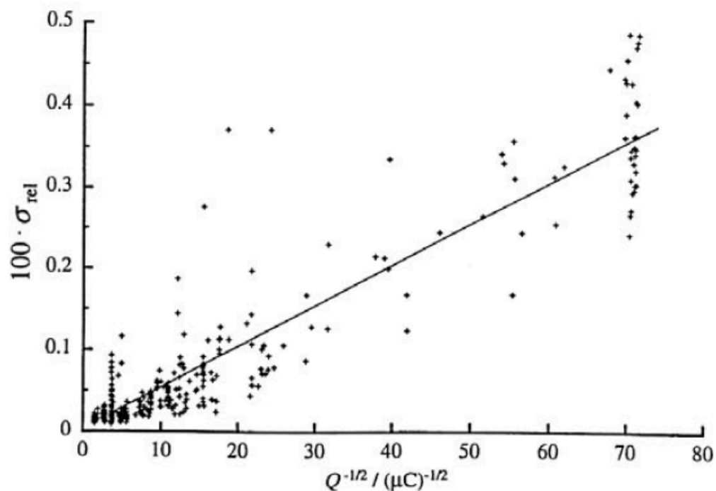
Figure 41-4 — Relative standard deviation \sigma_{\text{rel}} of repeated measurements in a series, with sources of variable activities plotted against Q^{-1/2} , where Q is the charge collected within the integration time for one measurement. Unpublished results from PTB (1992).
