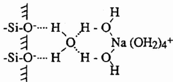
Figure 24 — Schematic representation of the interaction between the Na + ion and the surface probably taking place via hydrogen bonding between charged groups and solvated surface groups (Jolivet, 2000, see p. 54). Copyright (2000) John Wiley & Sons Limited. Reproduced with permission.
