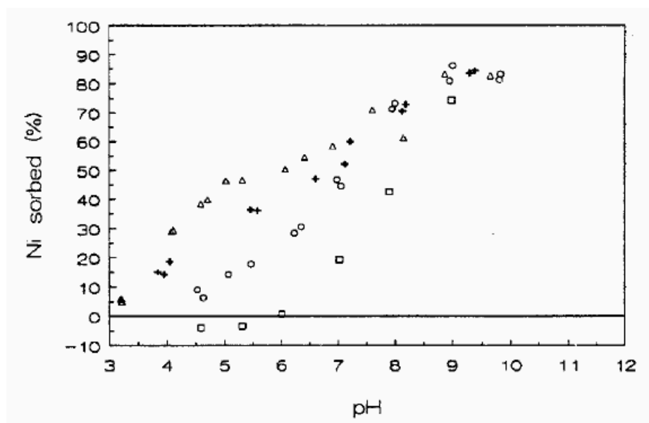
Figure 25 — Sorption isotherms for nickel Ni (II) on quartz (MUS (3) ) as a function of pH. System concentrations are: [Ni] = 5 \times 10^{-10} M and [SiO 2 = 60 "unitsml(g/L)". NaNO 3 medium concentrations are Δ 0.001 M; + 0.005 M; ○ 0.01 M; □ 0.1 M. From (Puukko and Hakanen, 1995, see p. 55) by permission.
