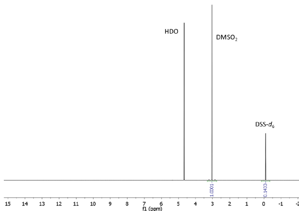
Figure A1.1 — 1 H NMR spectrum of DSS- d_6 and DMSO 2 in D 2 O.
