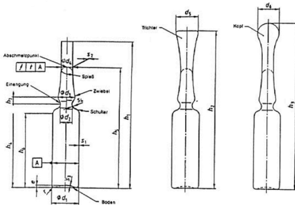
Figure 50-2 — Standard ampoules after ISO 9187-1:1991, Part 1, with dimensions to be standardized. (Abschmelzpunkt \Rightarrow sealing point, Spieß \Rightarrow spear, Einengung \Rightarrow embankment, Zwiebel \Rightarrow onion (-shape), Schulter \Rightarrow shoulder, Boden \Rightarrow bottom). Reproduced from ISO 9187-1:1991.
