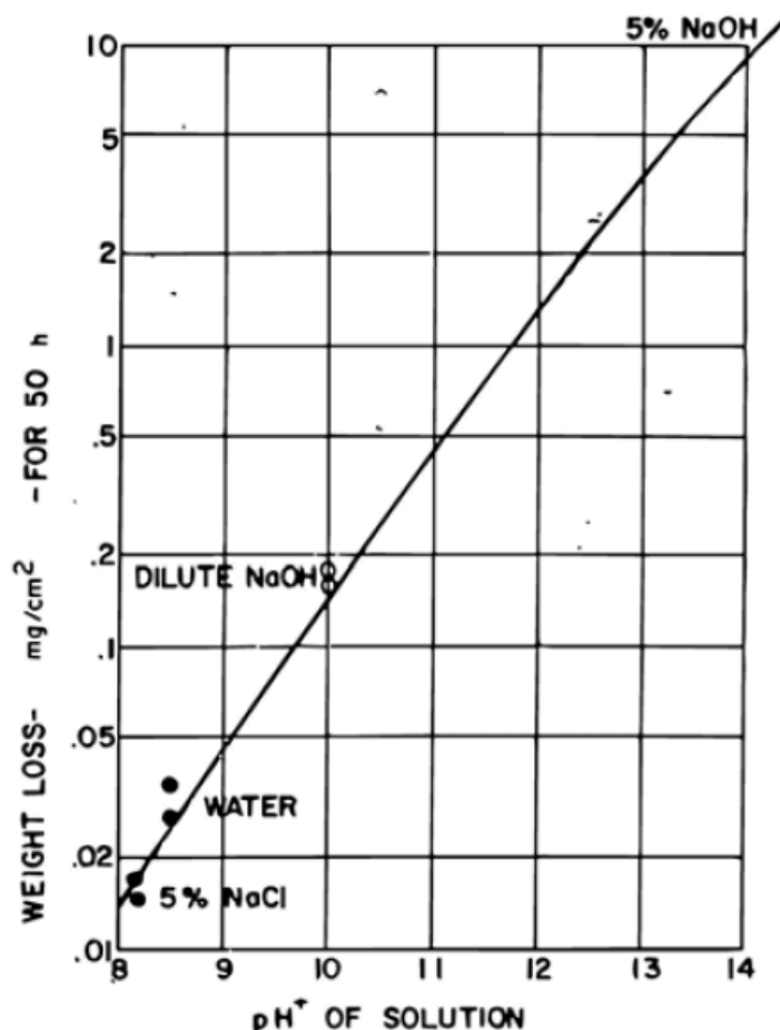
Figure 6 — Alkali attack of borosilicate glass in terms of mass loss ( \text{mgcm}^{-2} ), as a function of the pH of the reagent at 95 °C and a reaction time of 50 hours (Shand, 1958, see p. 55). Courtesy Corning Incorporated. Reprinted with permission.
