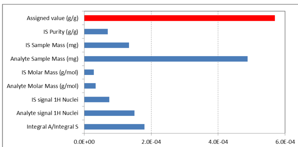
Figure A1.2 — Relative uncertainty components (in blue) for the uncertainty in the assigned purity value (in red) for MA using KHP as ISRM in \text{D}_2\text{O} .
