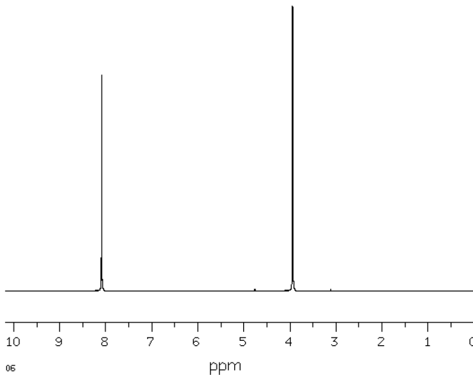
Figure 2 — ^1\text{H} NMR spectrum of DMTP in \text{CDCl}_3
