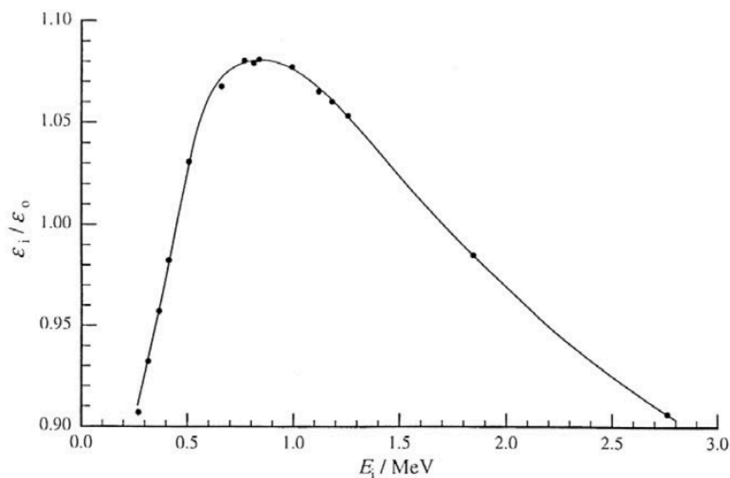
Figure 64-2 — Reduced efficiency curve. After Weiss ([470], see p. 194).
