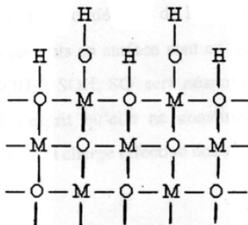
Figure 8-3 — Protons dissociate from the sorbed H 2 O molecules, leading to the formation of a uniformly hydroxylated surface.
