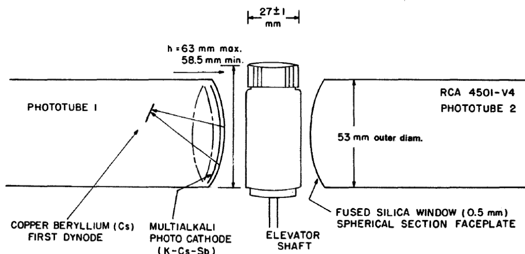
Figure 4 — Schematic diagram of standard counting vial and phototubes used for typical commercial LS counter (Packard TriCarb 3320).
