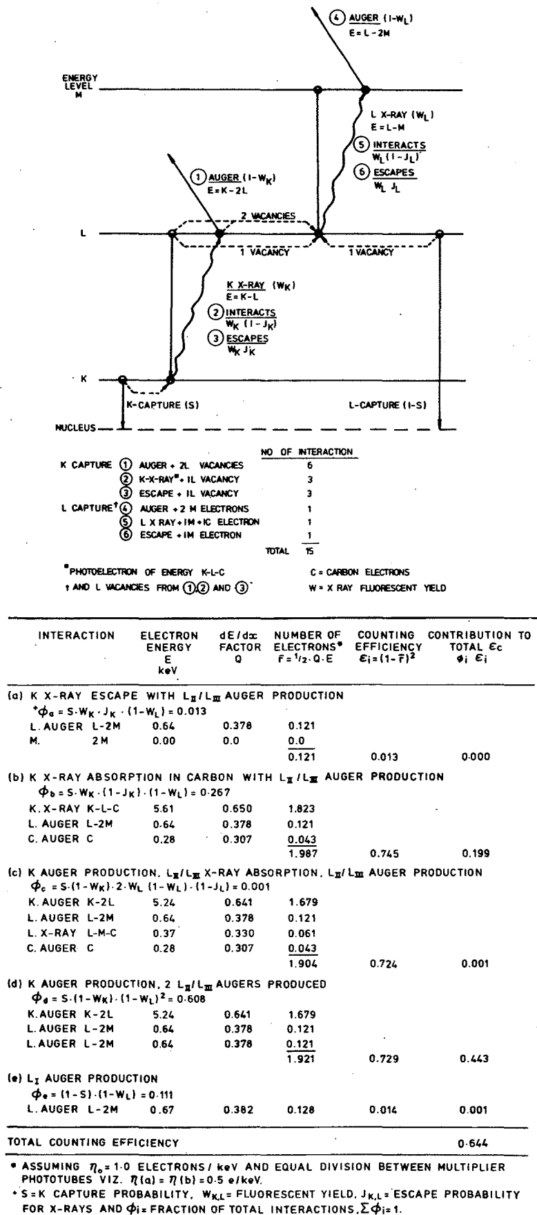
Figure 13 — Selected interactions for EC nuclides and a calculation of the efficiency for ^{55}\text{Fe} in a coincidence system at figures of merit of \eta_0 = 1.0 and 0.5 photoelectron/keV [195] (courtesy Pergamon Press Ltd., Oxford).
