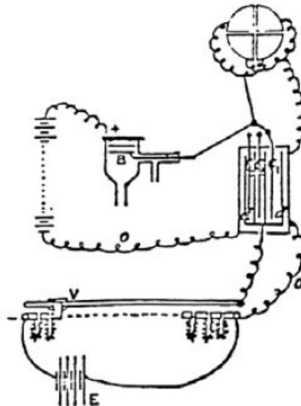
Figure 32 — Early induction balance from Townsend ([450], see p. 193) used for measurements "On the Genesis of Ions by the Motion of Positive Ions in a Gas", with the charge driven by the electric force from a battery (on left) and acquired by the plate B, a parallel plate condenser c; and d, the control instrument - an electrometer brought to zero by compensation - (on top of the figure), and the required compensation voltage V from a voltage divider of the voltage E, 0 giving the ground connections.
