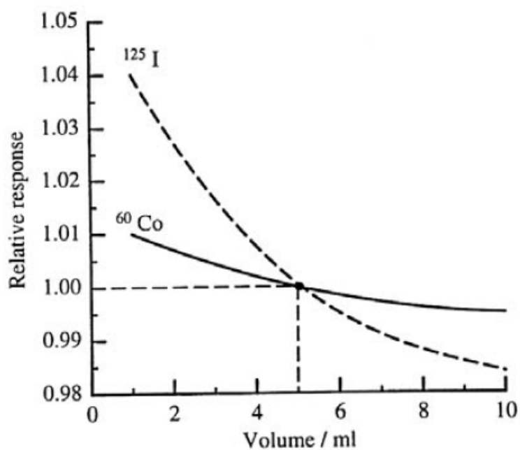
Figure 53-1 — Variation of ionization-chamber response with volume of solution relative to that of 5 ml volume (dashed line) for ^{60}\text{Co} and ^{125}\text{I} in a 10 ml P6 vial. After Woods et al. ([482], see p. 195).
