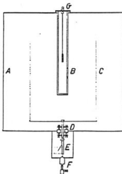
Figure 3-1 — Early re-entrant well ionization chamber with electrodes (A, B, C), amber insulator (D) and gold-leaf electrometer (E, F), source suspended on G, constructed by Bothe at the PTR in 1921. Reproduced from [153].
