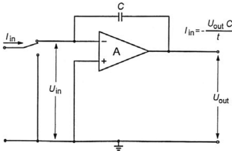
Figure 29-4 — Feedback-type current integrator, with feedback capacitor C .
