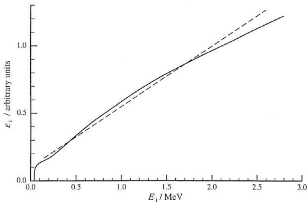
Figure 64-1 — Photon efficiency \varepsilon_1 versus photon energy for the PTB ionization chamber, type IG 12 of Centronic (see Figure 14, see p. 94). The dashed line shows the chosen linear efficiency function \varepsilon = 0.45 E + 0.1 for reduction (energy E in MeV). After Weiss ([470], see p. 194).
