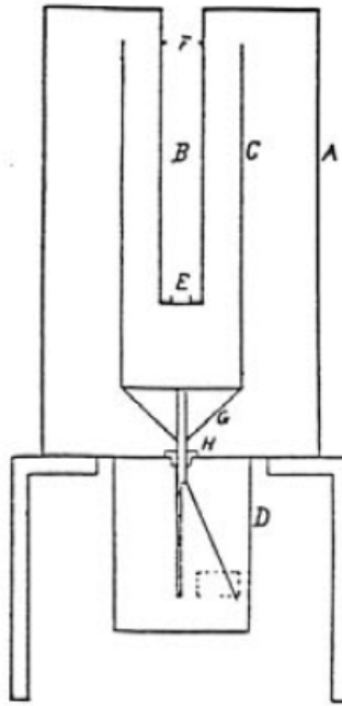
Figure 3-2 — Triple cylinder electroscope to measure sealed radium sources positioned at E within a re-entrant well (B) lined with lead. Reproduced from [117].
