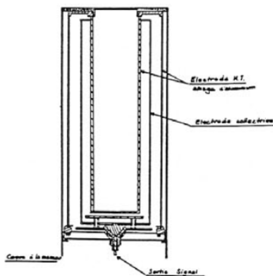
Figure 17-1 — Re-entrant ionization chamber used at LPRI, France.
