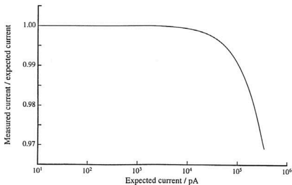
Figure 45 — Saturation loss characteristic for an ionization chamber developed at the NPL showing a break-down at very strong activities or corresponding large currents. After Woods et al. ([482], see p. 195).
