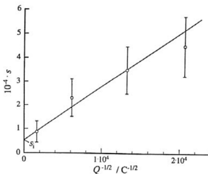
Figure 41-2 — Determination of the "internal" relative standard deviation s of repeated measurements, with sources of different activities, plotted against Q^{-1/2} , where Q is the charge collected within the integration time for one measurement. After Weiss ([469], see p. 194).
