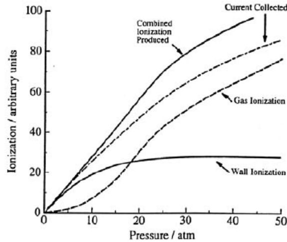
Figure 6 — Charge formation (ionization) and collection, with varying gas pressure in a highpressure ionization chamber with the two main components from the gas and the walls. After Boag ([30], see p. 166).
