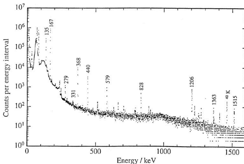
Figure 54 — Pulse-height spectrum of a ^{201}\text{Tl} solution source measured with a Ge-detector spectrometer to determine the activity parts of radionuclidic impurities such as in Table 3. (Ge-detector spectrum by PTB).
