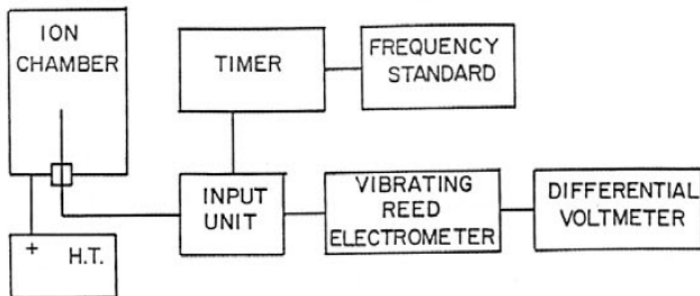
Figure 36-1 — Block diagram of the ionization current measuring system at the AECL, using the induction balance principle. The voltage difference across the capacitor of the input unit is measured by the vibrating-reed electrometer connected to a differential voltmeter during a given time interval.
