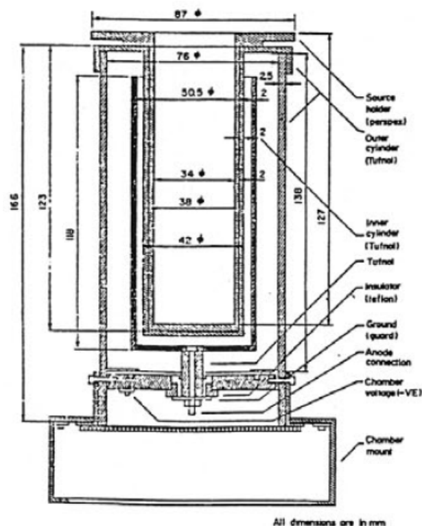
Figure 19 — Drawing of a radionuclide calibrator with a re-entrant air-equivalent chamber constructed from readily available plastic tube materials. A special conductive coating by colloidal graphite has been applied to the electrodes of the chamber. Reproduced from [386].
