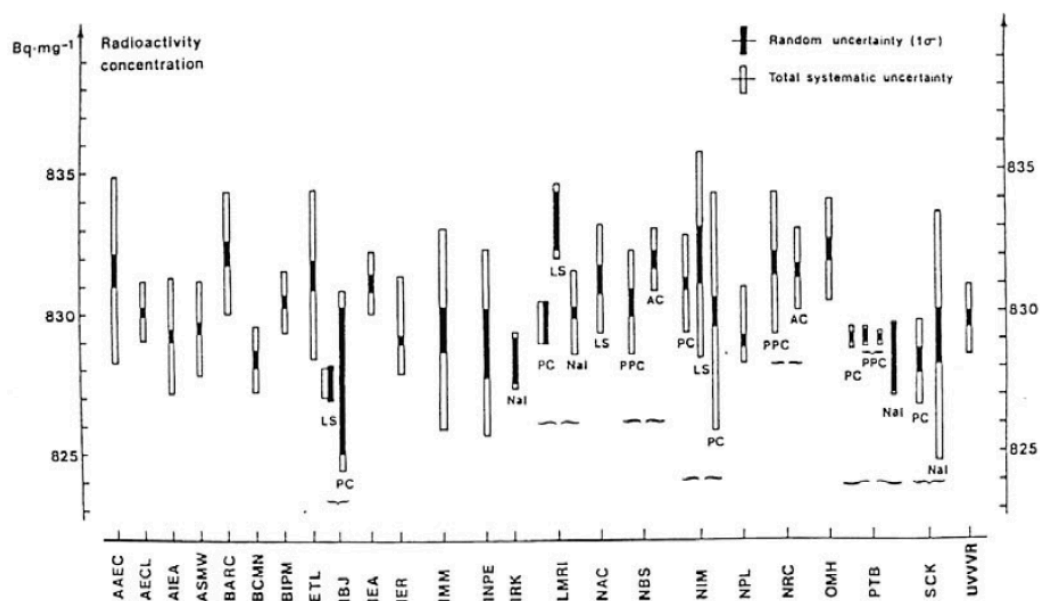
Figure 73 — Graphical representation of the results and their combined uncertainties (random and systematic effects) from a comparison of activity-concentration measurements with ^{134}\text{Cs} . The type of detector is indicated if a laboratory has submitted several results. Reproduced from [374].
