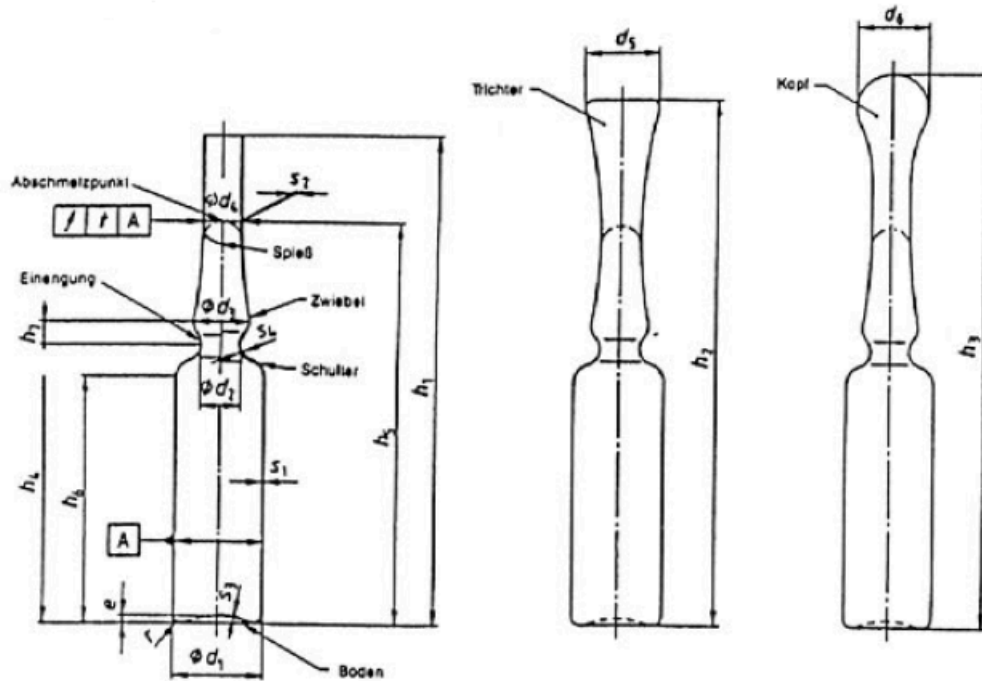
Figure 50-2 — Standard ampoules after ISO 9187-1, Part 1, with dimensions to be standardized. (Abschmelzpunkt \Rightarrow sealing point, Spieß \Rightarrow spear, Einengung \Rightarrow embankment, Zwiebel \Rightarrow onion (-shape), Schulter \Rightarrow shoulder, Boden \Rightarrow bottom). Reproduced from ISO 9187-1.
