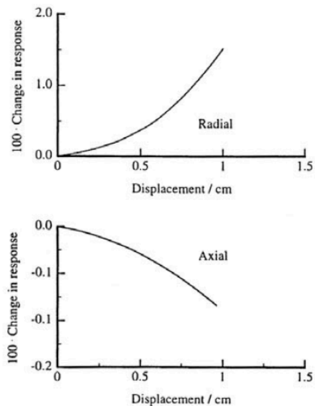
Figure 52-1 — Variation of response with displacement from the centre of an ionization chamber for 3 ml solution in 5 ml ampoule. After Woods et al. ([477], see p. 195).
