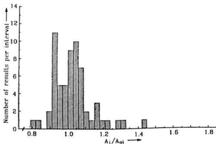
Figure 69-1 — Interval distribution for ^{99}\text{Tc}^m solution measured in glass vials.
