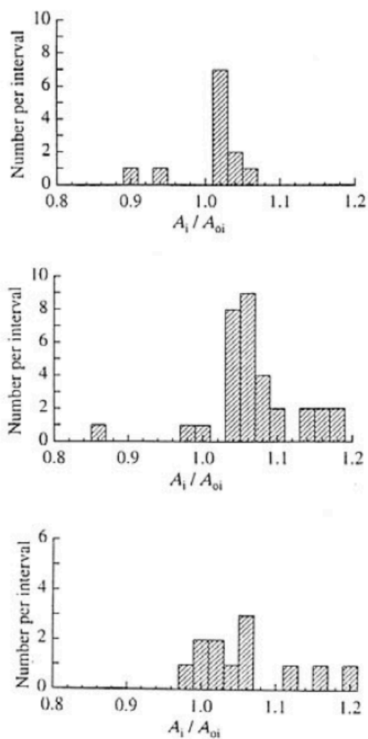
Figure 70-1 — For ^{57}\text{Co} solution measured in BS ampoules.
