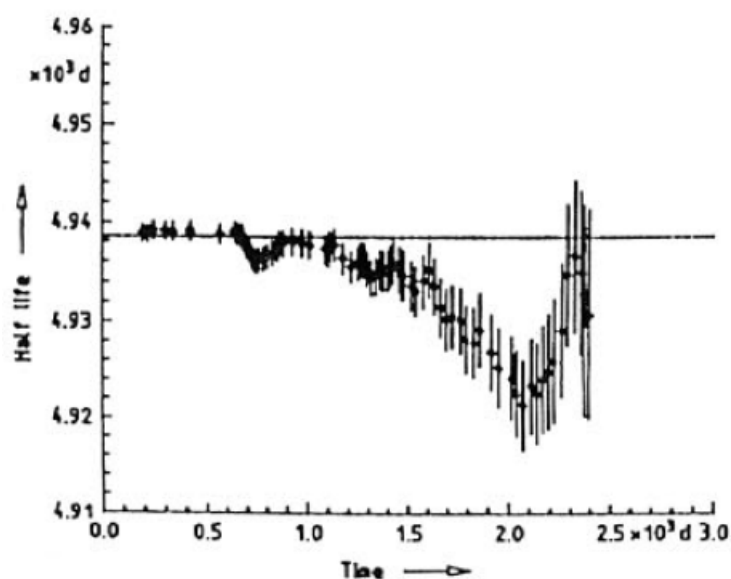
Figure 72-3 — Half-life values obtained starting from a data subset within the last 600 d and then, increasing the number in the subset by preceding data points successively (from right to left).
