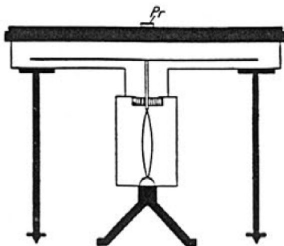
Figure 2-2 — Parallel-plate capacitor with electrometer to compare the activity of \gamma -ray emitting sources (Pr). After Curie ([87], see p. 170), reproduced from [260].
