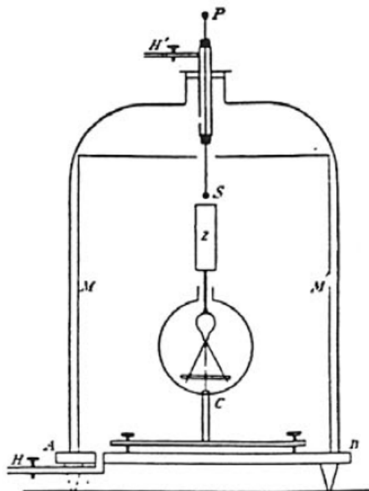
Figure 1-1 — Vessel with electrode (MM') and electroscope (Z) to study the "radioactive emanation" in air. Reproduced from [129].
