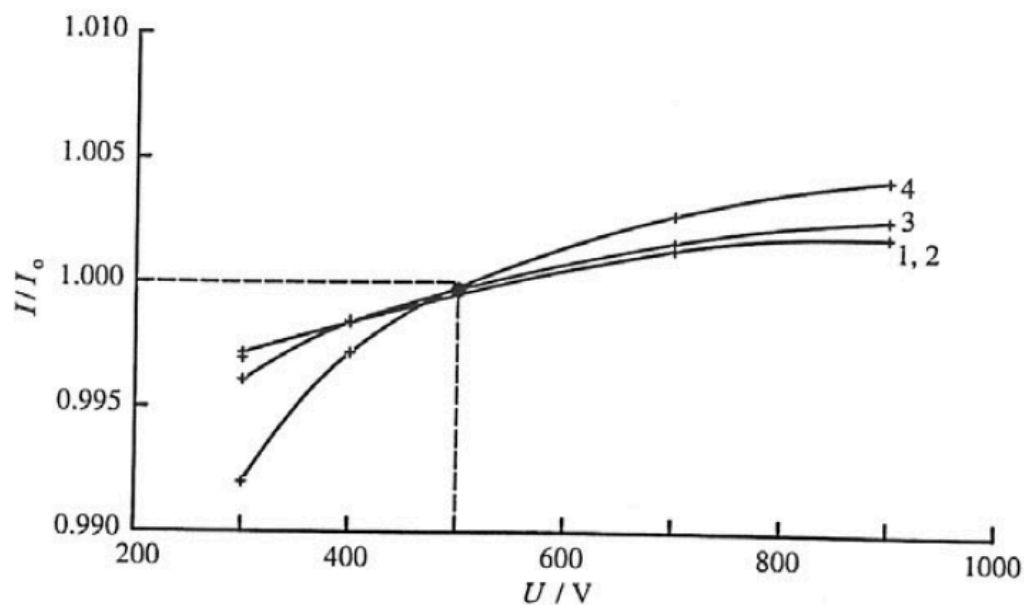
Figure 44-1 — Response characteristics for a chamber of good quality with a slope of 0.08% / 100 V at the nominal operating point, similar to the result from AECL in Figure 43-1.
