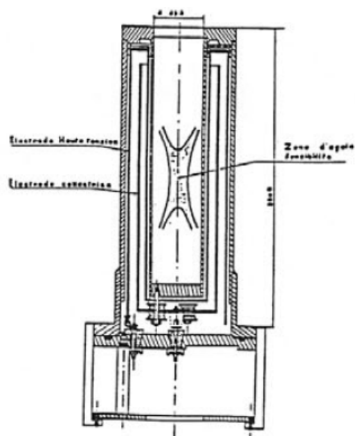
Figure 16 — Pressurized re-entrant ionization chamber filled with argon. The indicated zone in the well represents a cylinder of 4 cm diameter and 11 cm high with nearly constant efficiency values (variation within 1%). Reproduced from [187].
