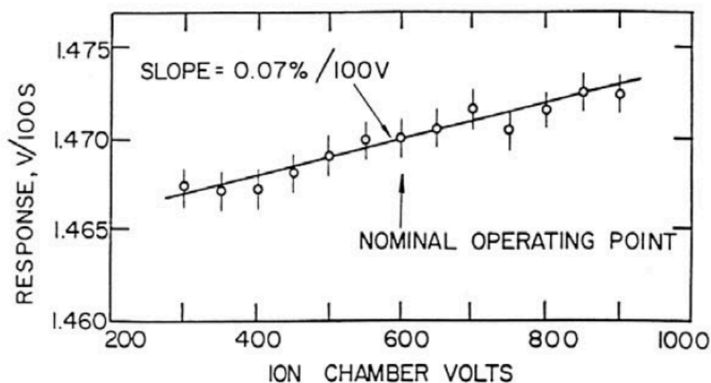
Figure 43-1 — Ionization chamber response for a source measured at various collection voltages applied between the electrodes, showing a slope of 0.07% / 100 V at the nominal operating point of the chamber (AECL, Chalk River). Reproduced from [307].
