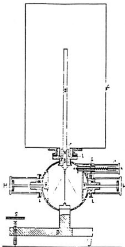
Figure 1-2 — Early ionization chamber (improved model of Figure 1-1 with a closed vessel). Reproduced from [131].
