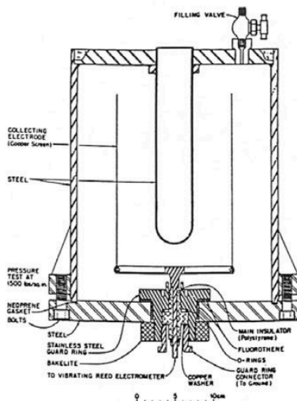
Figure 15 — High-precision, high-pressure ionization chamber by Shonka and Stephenson ([408], see p. 190). The chamber is filled with 40 atmospheres of dry argon. Reproduced from [326].
