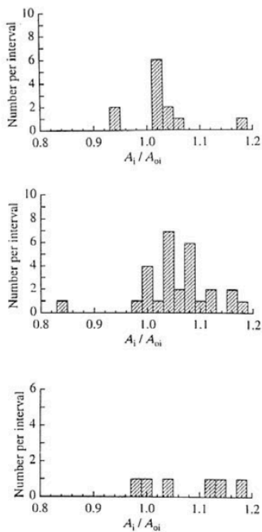
Figure 70-2 — For the same ^{57}\text{Co} solution measured in routine containers.
