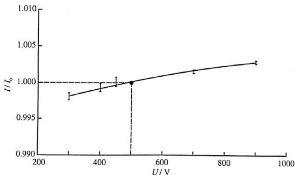
Figure 44-2 — Measurements in an ionization chamber of bad charge collection characteristics with rather large deviations from a flat linear slope for source no. 4. Unpublished results from the PTB (1987).
