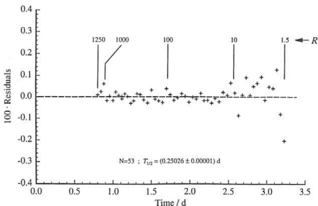
Figure 48-2 — For a reduced range of about eight times the ^{99}\text{Tc}^{\text{m}} half-life, data corrected for the ^{99}\text{Mo} impurity contributions. (Unpublished results, PTB).
