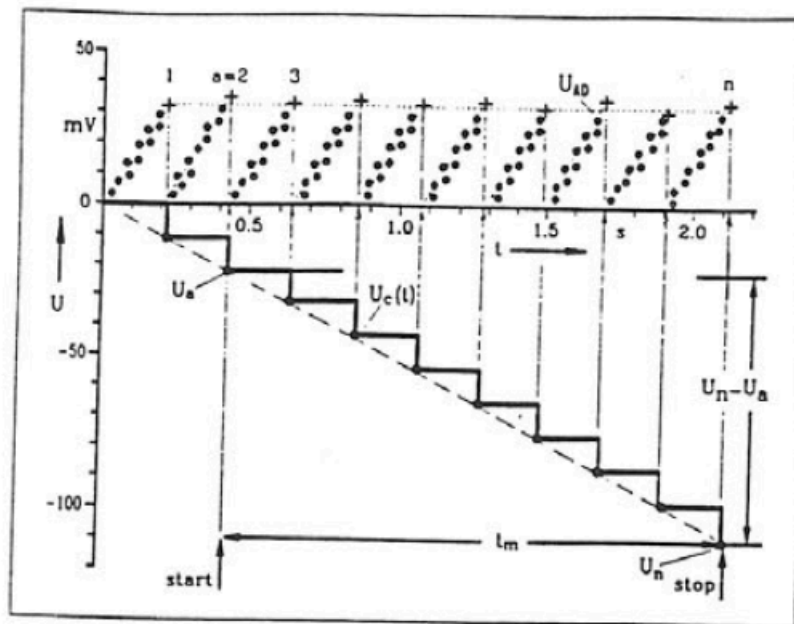
Figure 39-3 — Voltage-time diagram for the induction balance of Figure 39-2 showing n compensation steps during the measuring time t_m . U_{AD} is the voltage at the A/D converter input represented by circles. The crosses show the extrapolated U_{AD} values before a compensation step is transformed in the computer. U_C(t) is the resulting voltage at the D/A converter output which is fed to the capacitor represented by the step function. The measured ionization current is I = C(U_n - U_a)/t_m . Reproduced from [397].
