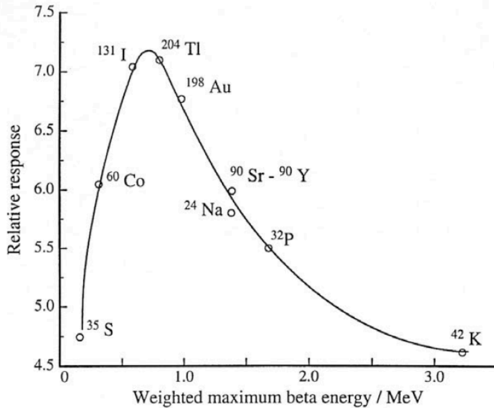
Figure 60-1 — Energy response of the NBS 2\pi\beta -ionization chamber. The current per unit activity has been plotted as a function of the maximum \beta -particle energy. The energy value is the weighted average of the energies of the branches when there is \beta -particle branching. The response curve appears to be a smooth curve on both sides of a peak at a maximum energy of approximately 0.7 MeV. The decrease above the peak is due to the finite dimensions of the chamber. Early data after Mann and Seliger ([295], see p. 183).
