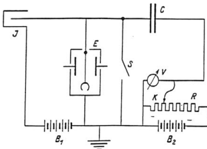
Figure 33-1 — Induction balance after Townsend ([450], see p. 193), with ionization chamber J , electrometer E , high tension on the chamber B_1 , voltage B_2 to create the compensating charge by shifting the contact K on the potentiometer R , precision voltmeter V , charge-collecting precision capacitor C and zero switch S .
