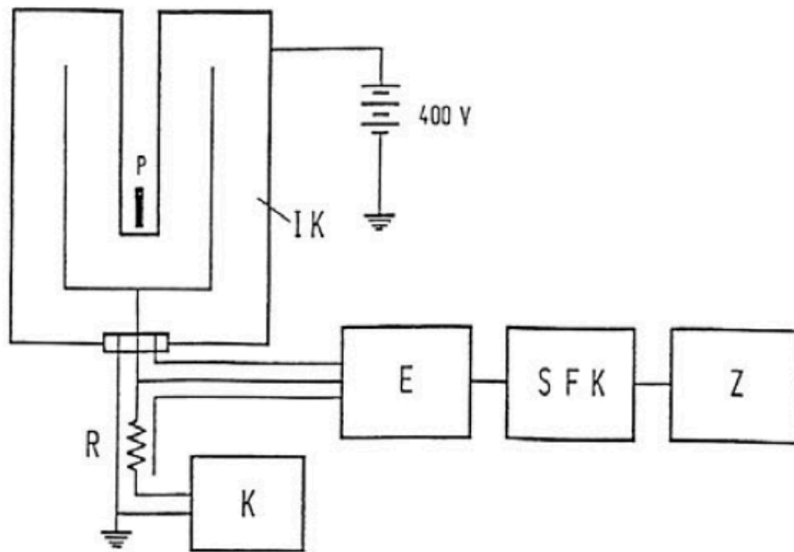
Figure 31 — High-ohmic resistor circuit for ionization current measurements from Walz and Weiss ([459], see p. 193), with radioactive source P, high-ohmic resistor R, vibrating-reed electrometer E, voltage compensator K, voltage-frequency converter SFK and counter chain Z.
