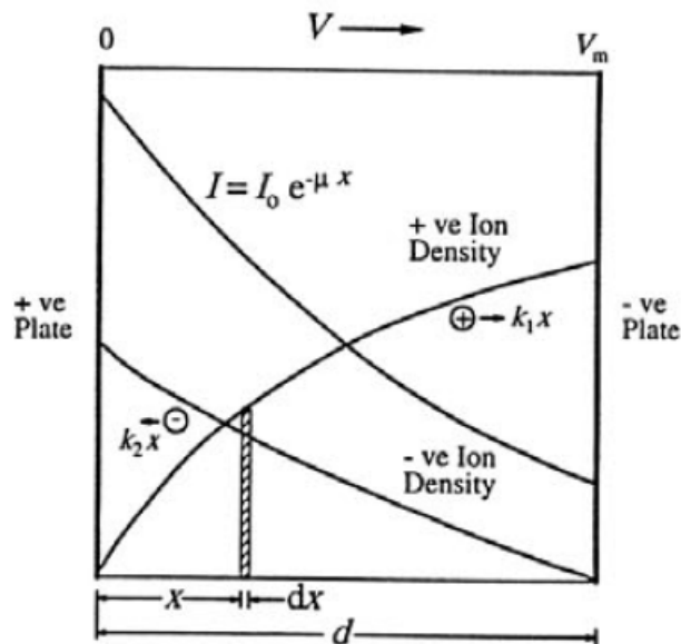
Figure 7 — Charge formation and density in a plane-parallel geometry chamber as a function of distance x measured from the electrode where the beam enters the gas space. I ionization intensity, \mu attenuation coefficient, k_1 and k_2 ionic mobilities, v collecting voltage and d distance between plates. After Boag ([31], see p. 167).
