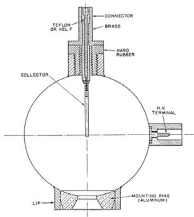
Figure 21 — Schematic drawing showing the construction of the 2\pi\beta -ionization chamber at NBS (NIST) with the source mounting at the base of the sphere. Reproduced from [403].
