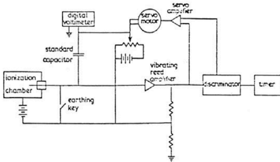
Figure 35-2 — Schematic diagram of an automatic induction balance with a servo-motor driven potentiometer for compensation at a charge-collecting standard capacitor. The control instrument coupled to the ionization chamber is a vibrating-reed amplifier with a discriminator for switching the servo-motor. The time during compensation is measured. Reproduced from [175].
