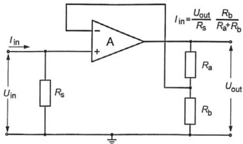
Figure 29-1 — Shunt-type picoamperemeter, with input resistor R_s and output voltage divider R_a, R_b .
