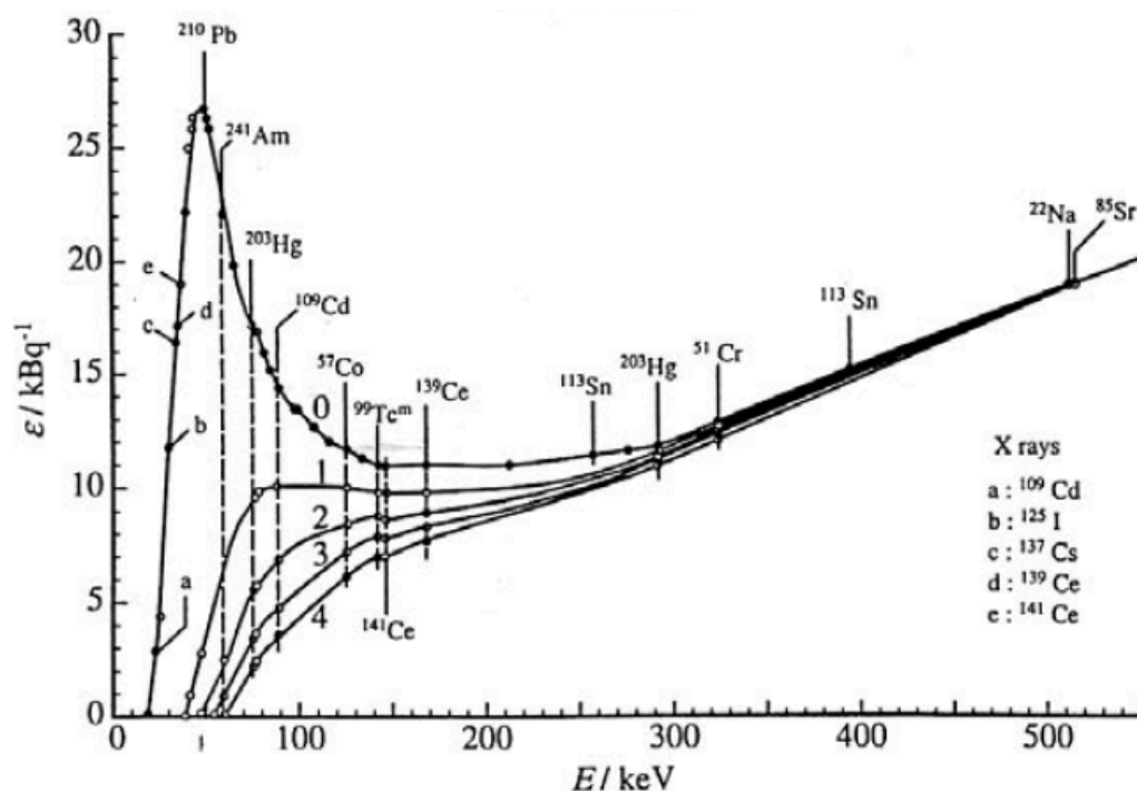
Figure 59 — Photon efficiencies \varepsilon versus photon energy E with various radionuclides for a radionuclide calibrator without and with Fe filters of various thickness around the source for photon energies from about 15 keV to 550 keV, without filter, marked by (0), and with Fe filter from 1 mm to 4 mm thick, marked by (1) to (4). (Unpublished data from PTB).
