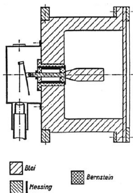
Figure 5 — Ionization chamber for external source positions with lead entrance window (Blei ⇒ lead, Messing ⇒ brass, Bernstein ⇒ amber). Reproduced from [264].
