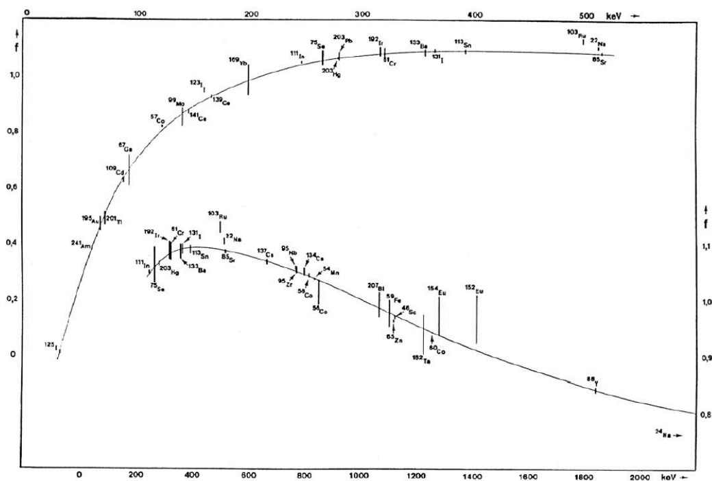
Figure 63-1 — Relative photon efficiency f of the ionization chamber of the SIR (BIPM) versus photon energy. The ordinate f is calculated relative to an arbitrarily chosen efficiency function which increases linearly with energy. The curve on the right gives the high energy part of the relative efficiency
