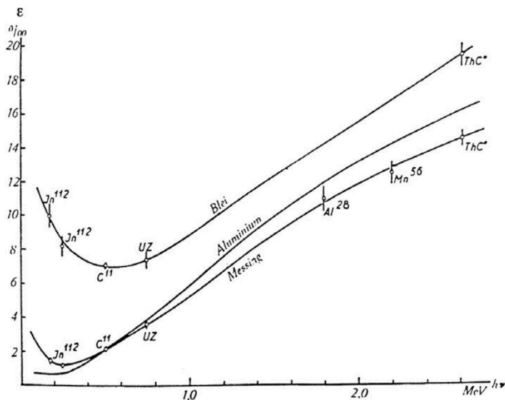
Figure 65-2 — Curves for tube materials such as lead, aluminium and brass (Aluminium \Rightarrow aluminium, Blei \Rightarrow lead, Messing \Rightarrow brass).
