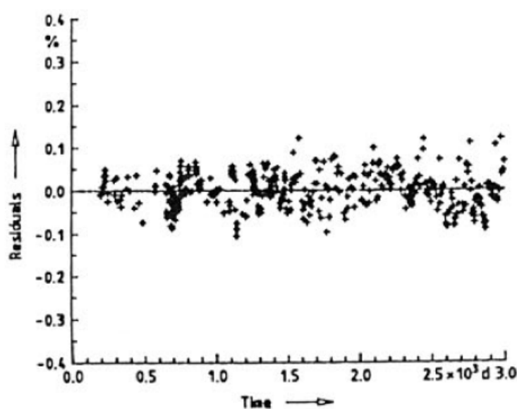
Figure 72-1 — Residuals for 384 data points measured during 2700 d giving a fitted half-life value of (4938.31 \pm 0.98) d.
