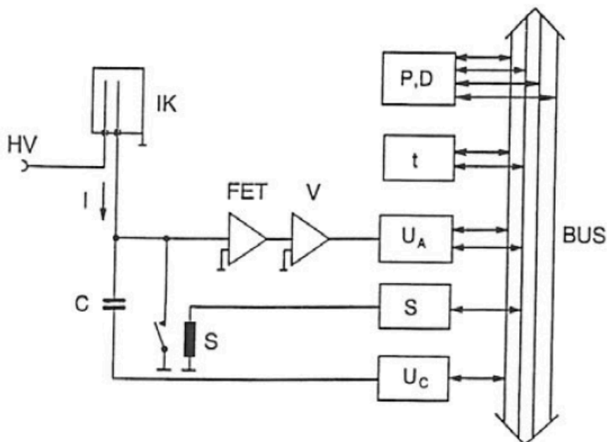
Figure 39-2 — Functional diagram of a current-measuring system by an induction balance, using a modified Townsend method with a capacitor C and a control loop for compensation with a programmable analog-digital (A/D) converter U_A and a digital-analog (D/A) converter U_C of high quality and resolution; other components as in Figure 39-1. Reproduced from [397].
