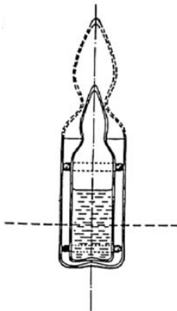
Figure 50-1 — Arrangement for an investigation of the influence of the ampoule walls. The small ampoule of BIPM/NBS(NIST) type contains a strong solution of ^{241}\text{Am} . The dashed top of a glass absorber has been cut off. The measurements were done with the SIR at the BIPM. Reproduced from [372].
