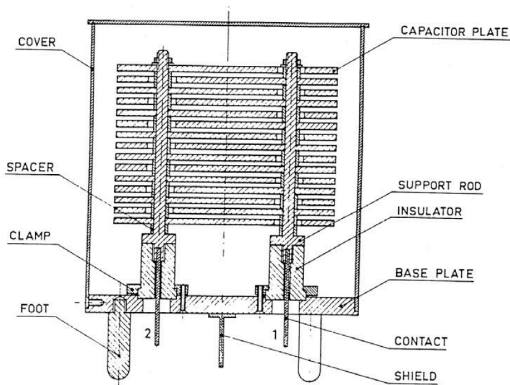
Figure 40 — Schematic view (vertical cut) of the 500 pF air capacitor used at the IRMM (CBNM), Geel. Reproduced from [353].
