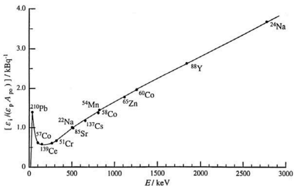
Figure 58-1 — Without filter up to a photon energy of 2754 keV.
