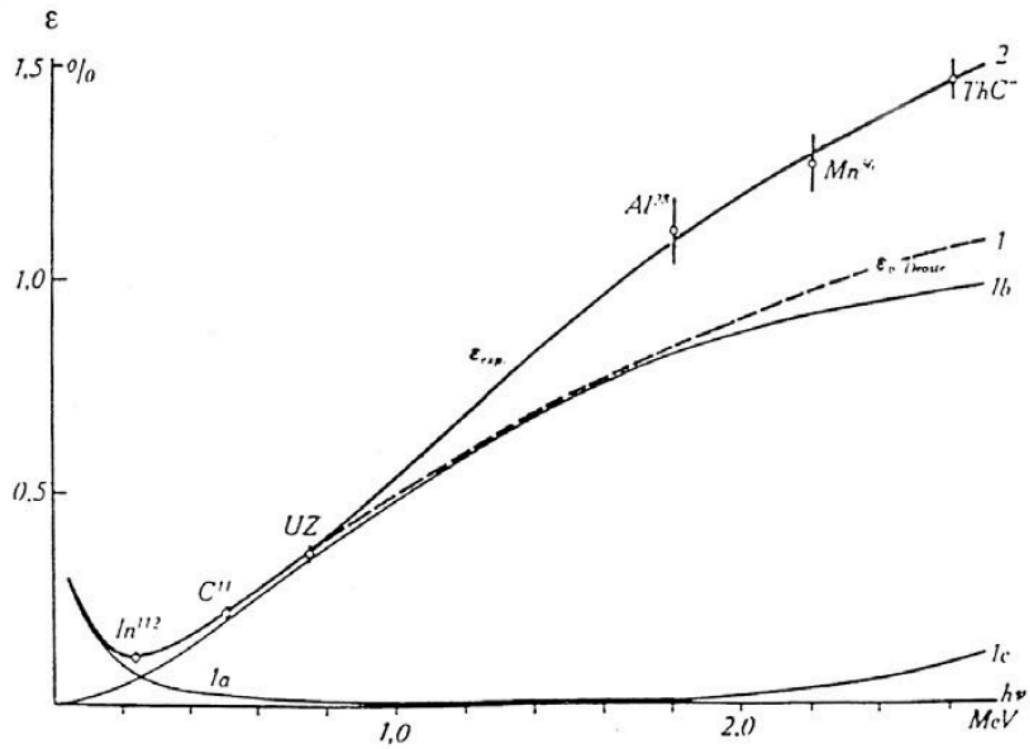
Figure 65-1 — Curve 1 is calculated for copper by the model of v. Droste ([118], see p. 172) using photon interaction with parts from photo effect (a), Compton effect (b) and pair creation (c), curve 2 is experimentally determined.
