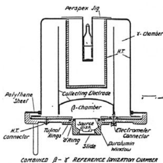
Figure 18 — Combined \beta - \gamma reference ionization chamber constructed at NPL. The ampoule position with \gamma -ray emitting solution is shown in the perspex jig, a \beta -particle emitting source may be placed on the source dish in the bottom of the chamber below a thin duralumin entrance window [355]. The sensitivity of this chamber was studied in detail by Dale et al. ([91], see p. 170). Reproduced from [316].
