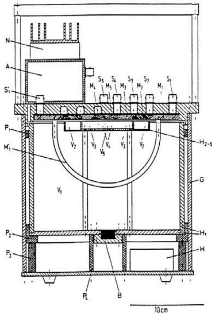
Figure 26 — Sectional drawing of a reference current source using the ionization from \beta radiation (B) with sensitive volumes V_j and electrodes M_j and H_j (high tension), connected via the plugs S_j to an amplifier A and electronics N. P_j and G are housing materials. Reproduced from [36].
