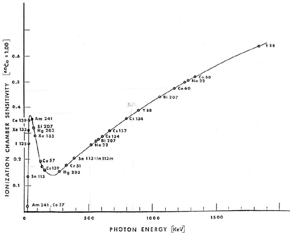
Figure 62 — Sensitivity of typical ionization chamber of calibrator as a function of photon energy. Sensitivity is normalized by chamber response to ^{60}\text{Co} radiations. Reproduced from [431].
