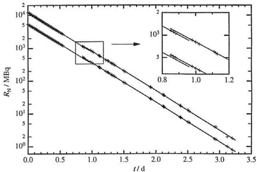
Figure 47-1 — Decay curves of two ^{99}\text{Tc}^{\text{m}} sources in a logarithmic plot.
