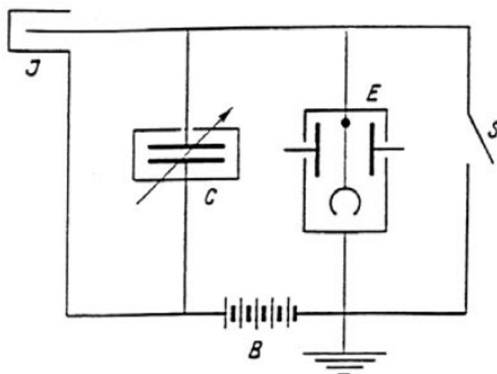
Figure 33-2 — Compensation by varying a calibrated capacitor C with ionization chamber J , electrometer E , high tension B on the chamber and zero switch S .
