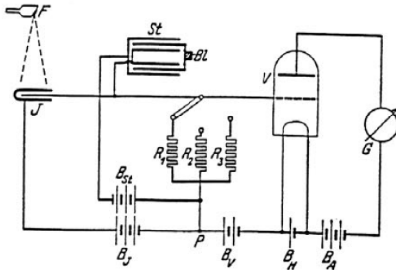
Figure 33-3 — Compensation by an adjustable current source St(BI) , with ionization chamber J , vacuum-tube entrance stage V on the measuring instrument G , high tension on the chamber B_J , high-ohmic resistors R_i for range switching and voltage supplies B_i for the various components. This represents an early application of a vacuum tube with an x-ray dosimeter by Siemens.
