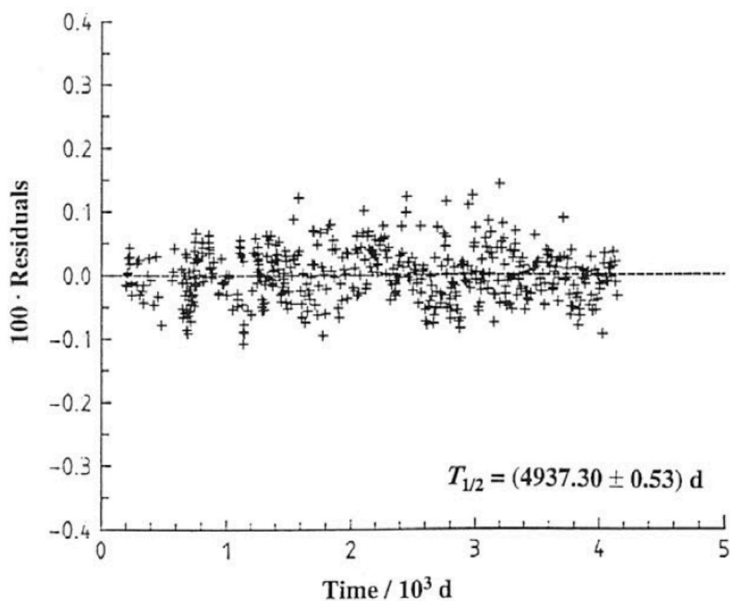
Figure 71-1 — Residuals for 557 data points measured during 3950 d giving a half-life value of (4937.30 \pm 0.53) \text{ d} .
