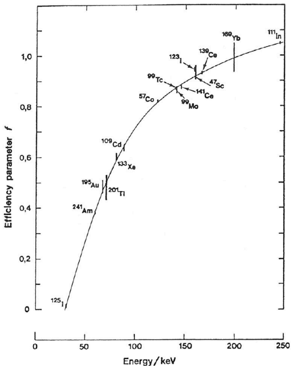
Figure 63-2 — Efficiency as a function of photon energy - updated low energy part of the curve of Figure 63-1 - for the SIR ionization chamber at the BIPM. Reproduced from [346].
