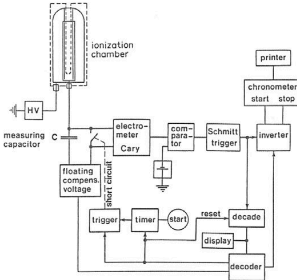
Figure 37-2 — Block diagram of the measuring electronics of the SIR (BIPM), based on the induction balance principle, with stepwise compensation and a preset voltage level. The time is measured for a well-defined number of compensation steps. Reproduced from [376].
