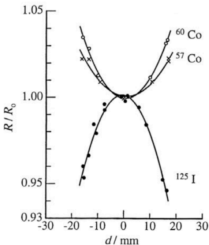
Figure 52-3 — Variation of a radionuclide-calibrator reading R/R_0 , normalized to that of the standard operating position for ^{60}\text{Co} , ^{57}\text{Co} and ^{125}\text{I} . The low-photon energy emitting source of ^{125}\text{I} shows a negative characteristic. Horizontal displacement. After Schrader ([398], see p. 190).
