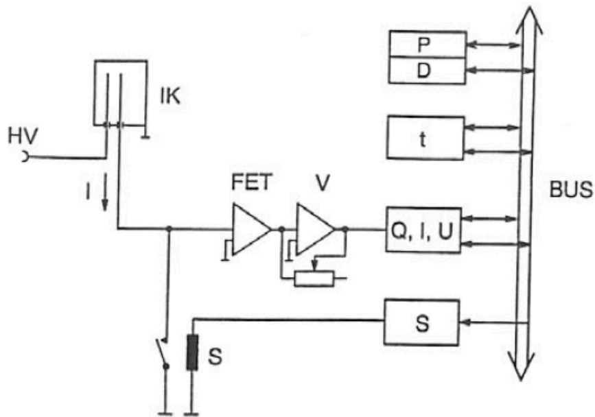
Figure 39-1 — Schematic diagram of a current-measuring system for an ionization chamber IK, with an FET-amplifier input V and programmable components connected to a computer bus: P, D processor and instrument display, t timer, Q, I, U measurement components for charge, current or voltage to be chosen and S switch to ground potential. Reproduced from [398].
