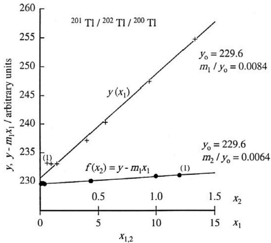
Figure 55-2 — For a ^{201}\text{Tl} source with two radionuclidic impurities; the admixture of ^{202}\text{Tl} is first analysed in the presentation of y(x_1) , indicated by crosses, and then, ^{200}\text{Tl} in y - m_1 x_1 , indicated by dots. The x_1 and the x_2 scale differ by a factor of 10.
