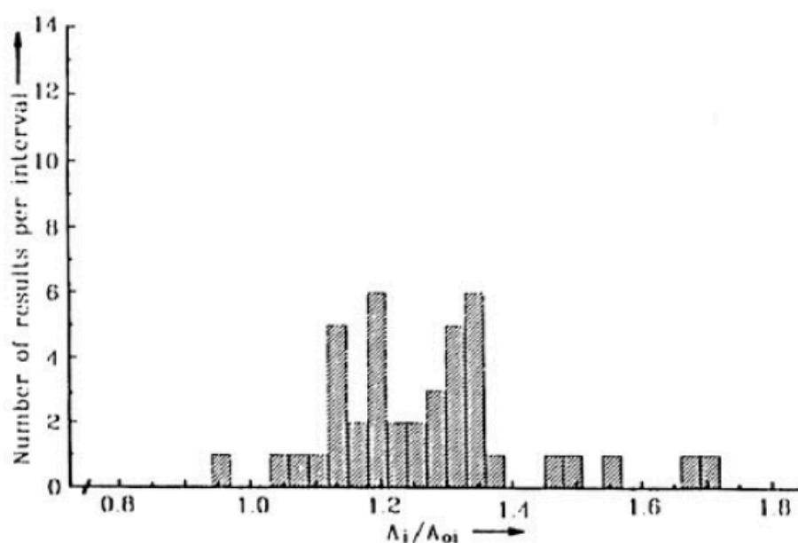
Figure 69-4 — Interval distribution of the same ^{123}\text{I} solution measured in a syringe and corrected for the residual activity.
