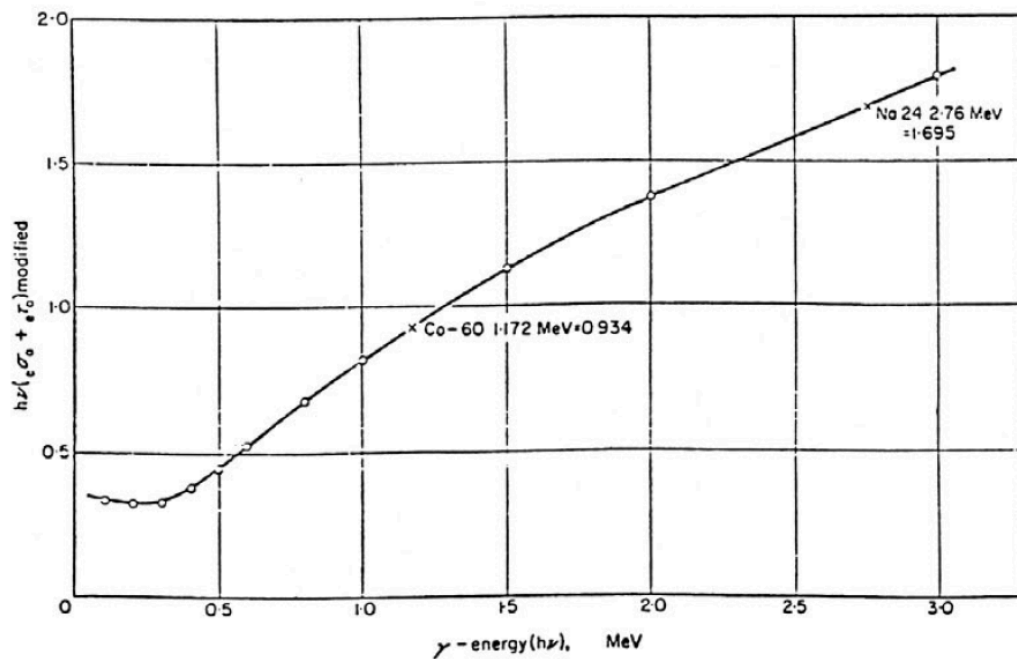
Figure 61-2 — Secondary electron production in brass against \gamma energy (modified for absorption in a brass liner of an ionization chamber cavity). Two radionuclides were selected, namely, ^{60}\text{Co} and ^{24}\text{Na} , from which it was hoped to normalize the curve so as to read directly in current I per \gamma -ray quantum against \gamma energy, and to calculate a response by simple summing of the contributions of the constituent \gamma rays of a radionuclide. Reproduced from [90].
