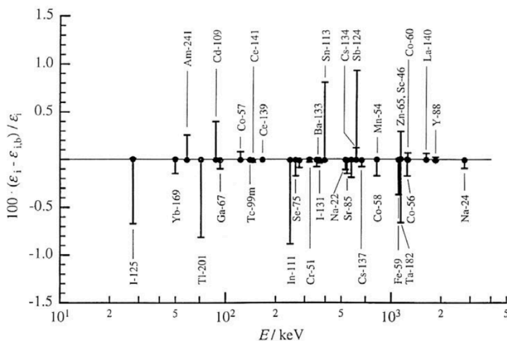
Figure 66 — Consistency check for the photon efficiency curve of the PTB ionization chamber. The radionuclide efficiency values were calculated in term of the weighted average of the corresponding photon efficiencies from the
