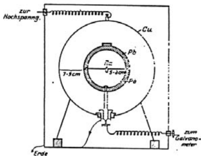
Figure 2-1 — Early spherical ionization chamber with a Ra source inside (zur Hochspannung \Rightarrow to high-tension, Erde \Rightarrow earth, ground potential, zum Galvanometer \Rightarrow to galvanometer). After Meyer and Hess ([308], see p. 184), reproduced from [260].
