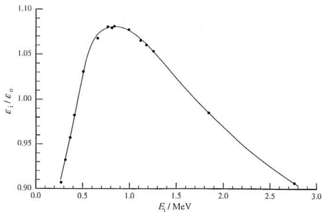
Figure 64-2 — Reduced efficiency curve. After Weiss ([470], see p. 194).
