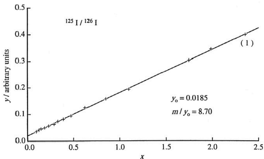
Figure 55-1 — For a ^{125}\text{I} source with a radionuclidic impurity of ^{126}\text{I} .
