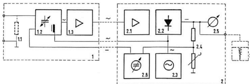
Figure 27 — Diagram of a vibrating-reed electrometer (VRE), with the capacitor modulator (1.2) generating an alternating voltage, a preamplifier (1.3) and amplifier (2.1) connected to a phase-related rectifier (2.2), which is controlled by the oscillator (2.3) driving the capacitor modulator synchronously. At the amplifier output an adjustable (2.4) compensation
