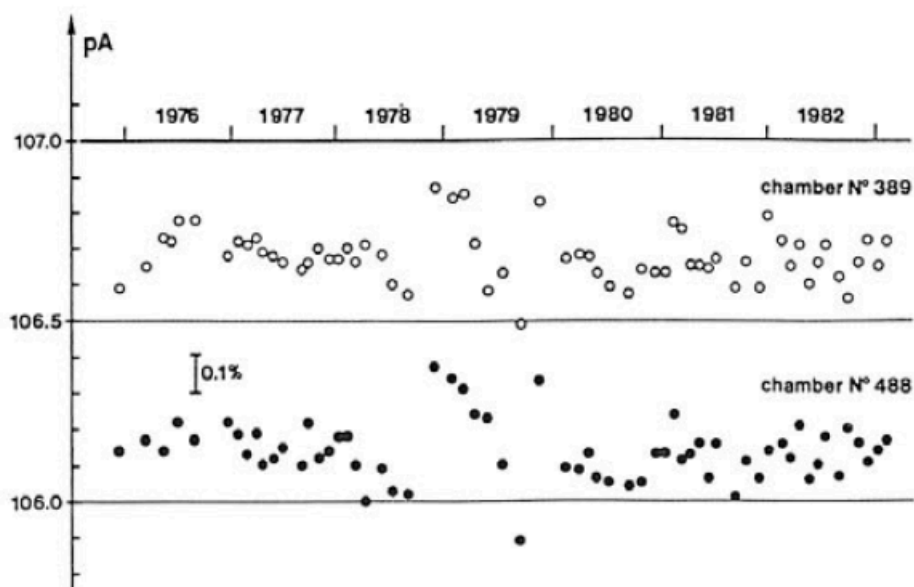
Figure 10-2 — Periodic measurements of the ionization current produced by reference source no. 2, placed in either of the two chambers of the SIR. Reproduced from [376].
