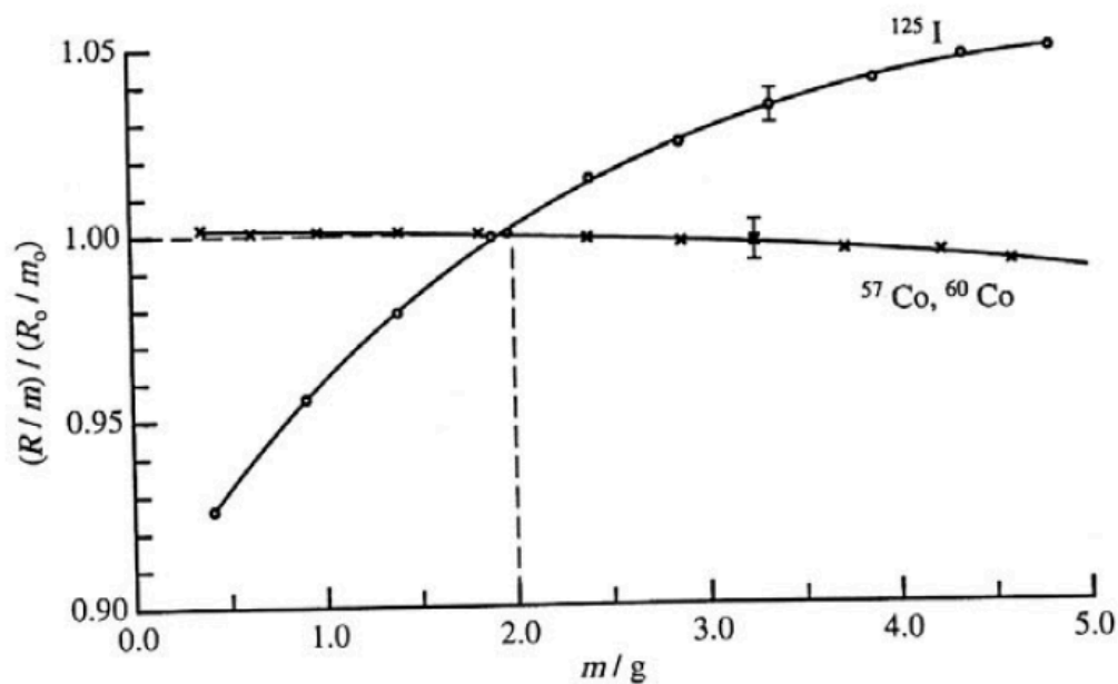
Figure 53-3 — Variation of instrument reading per solution mass \frac{R/m}{R_0/m_0} , normalized to that of a standard filling of m_0 = 2 g in a PTB ampoule: For the PTB ionization chamber, type IG 12 of Centronic (see Figure 14, see p. 94) with m_0 = 2 g (dashed line) and various photon-emitting radionuclides with energies above 120 keV. (Unpublished results, PTB).
