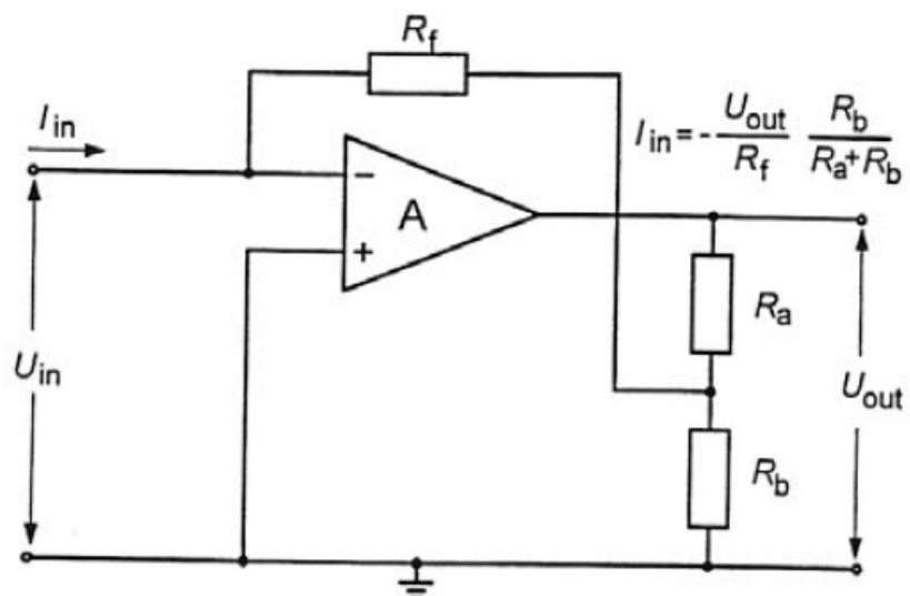
Figure 29-2 — Feedback-type picoamperemeter, with feedback resistor R_f .
