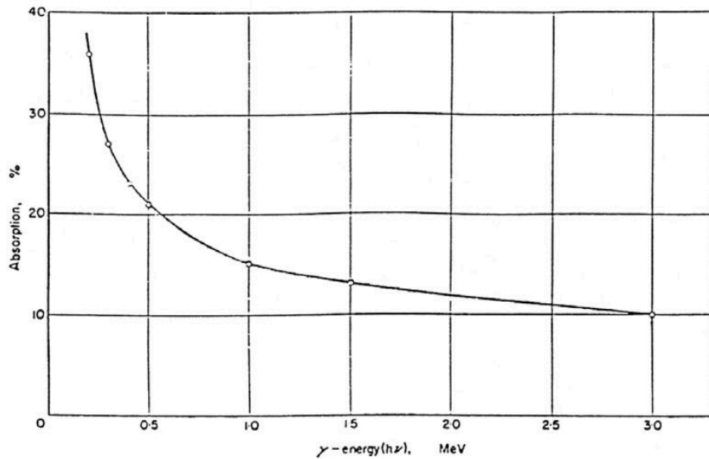
Figure 61-1 — Absorption of \gamma radiation in a brass liner of an ionization chamber cavity. Reproduced from [90].
