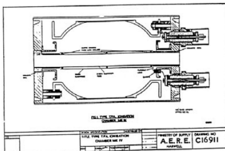
Figure 12 — Drawing of the TPA type Mk IV ionization chamber at AERE, Harwell, UK., constructed with thin aluminium walls and filled with argon to a pressure of one atmosphere. Reproduced from [458].
