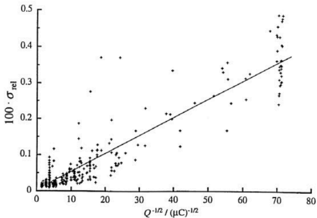
Figure 41-4 — Relative standard deviation \sigma_{\text{rel}} of repeated measurements in a series, with sources of variable activities plotted against Q^{-1/2} , where Q is the charge collected within the integration time for one measurement. Unpublished results from PTB (1992).
