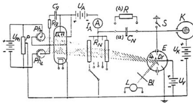
Figure 34 — Electrometer-photocell compensator by Hübner ([222], see p. 178), with ionization chamber K and high tension U_k . The electrometer E with a turning light-mirror system ( L , BI , Dr ) initiates variable currents on the photocells Ph_1 and Ph_2 connected to the vacuum tube EL11 , which itself controls the potential at point (a) by the voltage decrease on the high-ohmic resistor R_N and creating the compensation charge on the collecting capacitor C_N , for zero switch S open. The anode current I_{Ai} of the tube is measured by the instrument A during the time t at the beginning and the end of the compensation giving the ionization current
