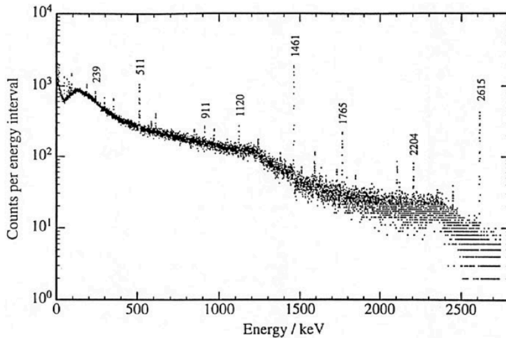
Figure 49 — Pulse-height spectrum of the natural background taken with a Ge-detector spectrometer in a typical environment for ionization chamber measurements. (Unpublished results, PTB).
