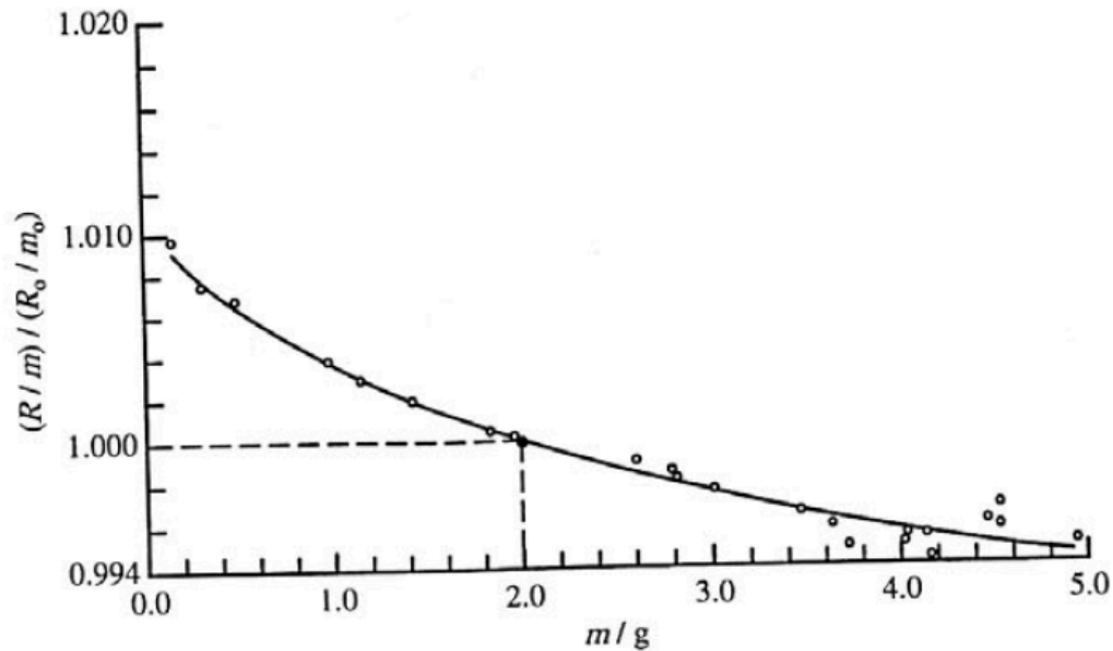
Figure 53-2 — Variation of instrument reading per solution mass (R/m)/(R_0/m_0) , normalized to that of a standard filling of m_0 = 2 g in a PTB ampoule: For a radionuclidecalibrator and ^{60}\text{Co} , ^{57}\text{Co} and ^{125}\text{I} . From Schrader ([398], see p. 190).
