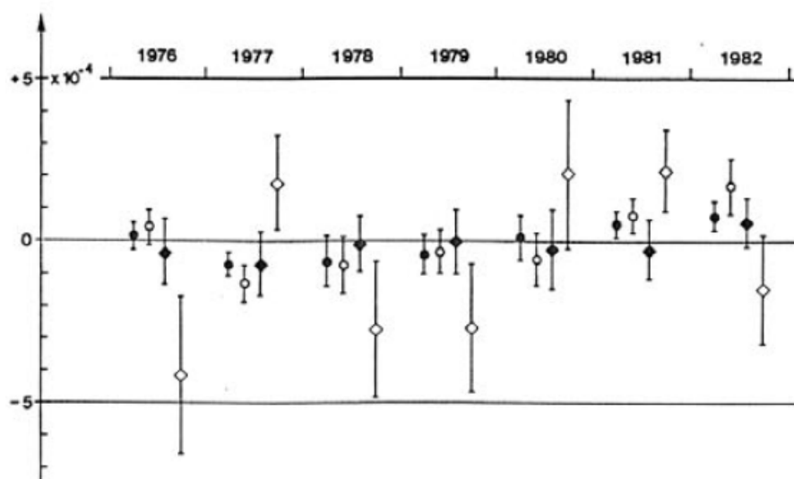
Figure 10-1 — Mean values and their uncertainties derived from periodic measurements of the ratios of reference sources no. 1 to 5, with relative deviations from the general mean for the SIR. • nos. 5/4, o 4/3, ♦ 3/2 and ◇ 2/1, respectively. Reproduced from [376].
