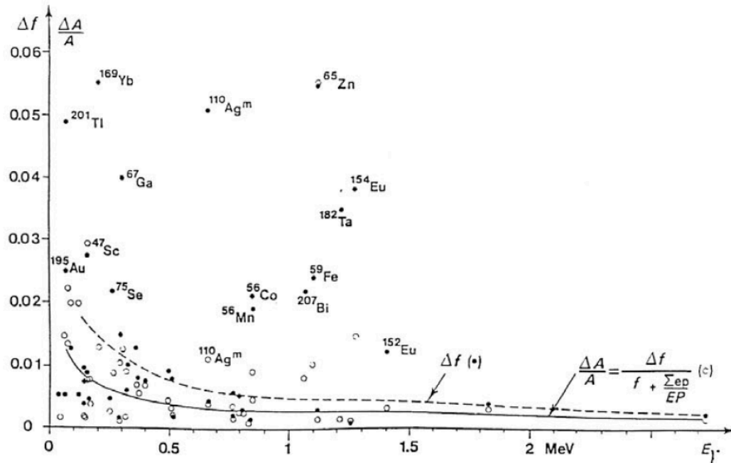
Figure 67 — Uncertainty of the measurements with the ionization chamber of the SIR (BIPM). The values of the deviation \Delta f (full dots and dashed line) calculated by the error propagation law from the uncertainty components of the reduced efficiency function f and the relative uncertainty of an activity measurement \Delta A/A (circles and full line) estimated from f are plotted versus photon energy E . Radionuclides showing larger deviations are referred. Reproduced from [378].
