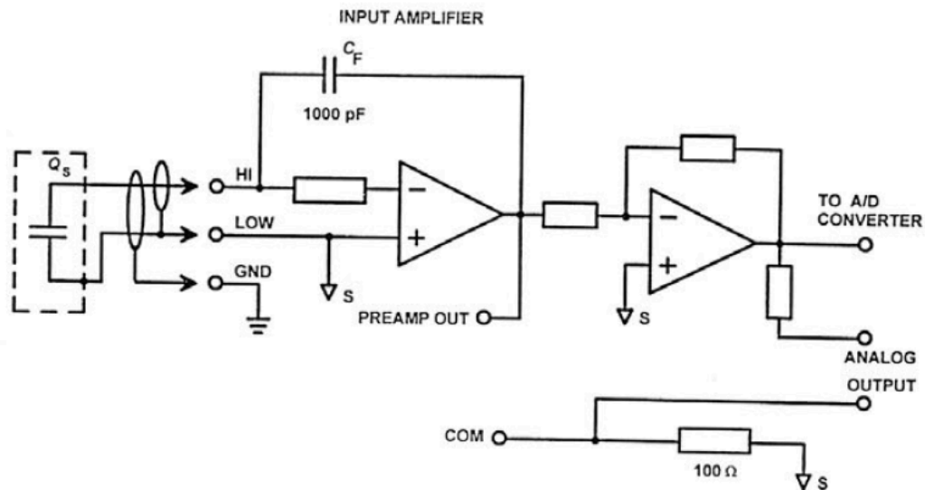
Figure 28 — Diagram of an electrometer with an FET-entrance stage, used for measurement ranges as low as 10^{-14} C. The charge source Q_s is connected by a triax cable to the FET preamplifier, with the feedback capacitor C_F working as an integrator, and via an amplifier to an A/D converter of a voltage instrument with digital display. After Keithley ([249], see p. 180).
