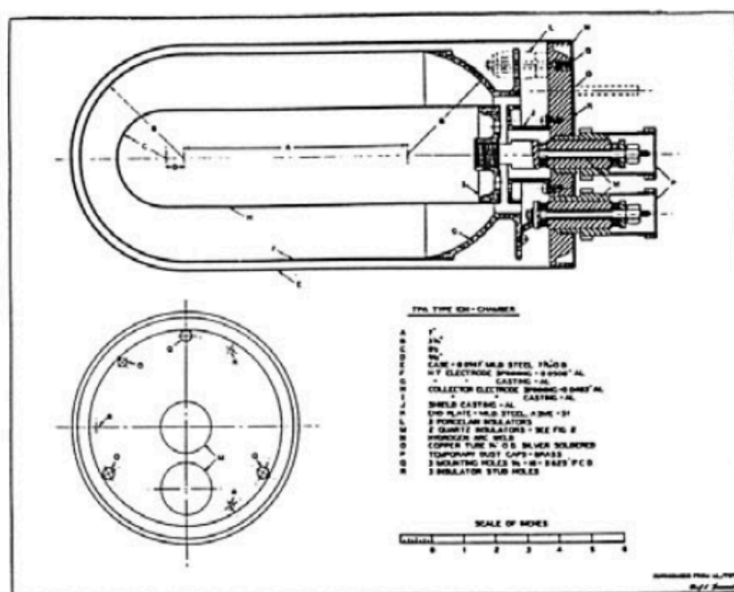
Figure 11 — Scale drawing of the TPA type ionization chamber at AECL (Chalk River). The chamber is tested to be filled with a gas up to a pressure of 20 atmospheres. Reproduced from [65].
