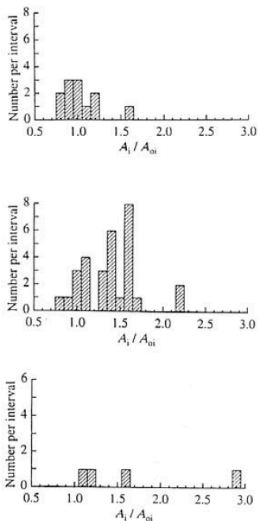
Figure 70-4 — For the same ^{125}\text{I} solution measured in routine containers.
