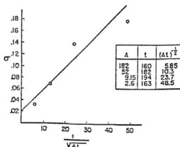
Figure 41-1 — Plot of the relative standard deviation \sigma of individual current measurements made on four radium sources, with activities from 3 \mu\text{Ci} to 200 \mu\text{Ci} , as a function of the total number of ions collected per radium source. Reproduced from [164].
