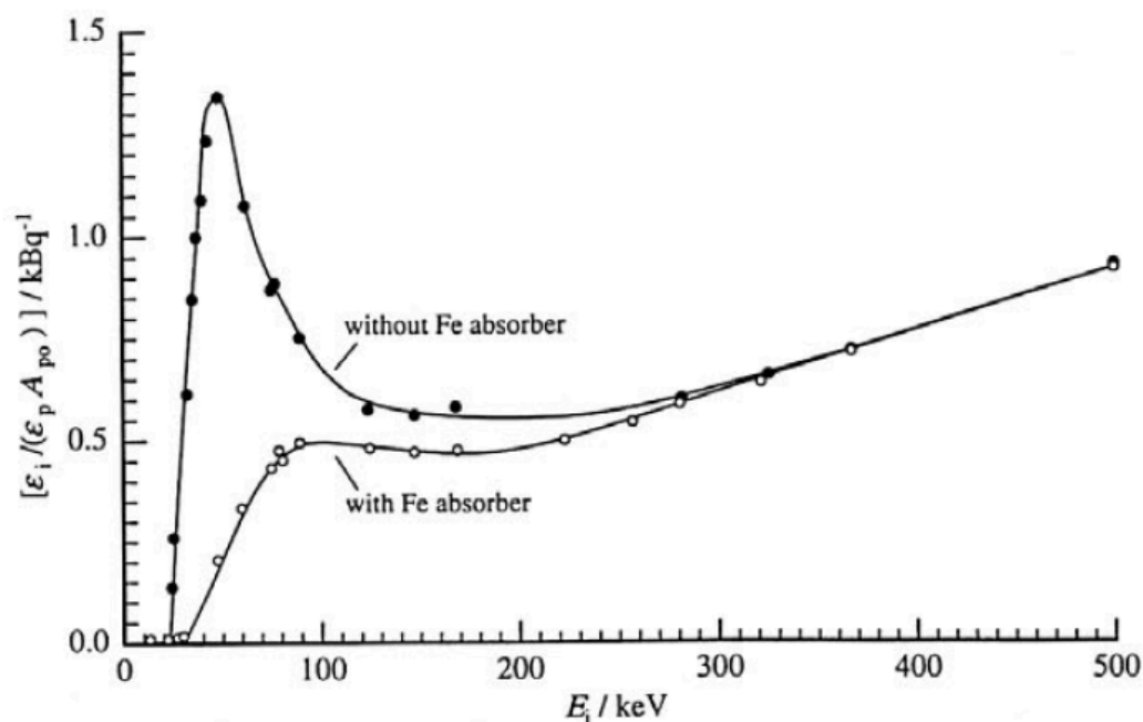
Figure 58-2 — Without and with Fe filter 1 mm thick and for photon energies from about 15 keV to 550 keV.
