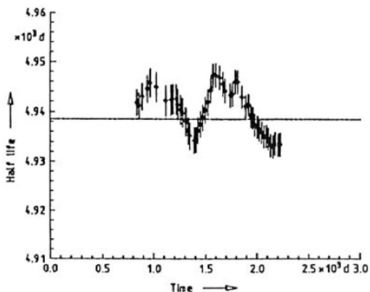
Figure 72-4 — Half-life values obtained from subsets of 200 points which were formed by a shift in the total set with steps of 5 data points each.
