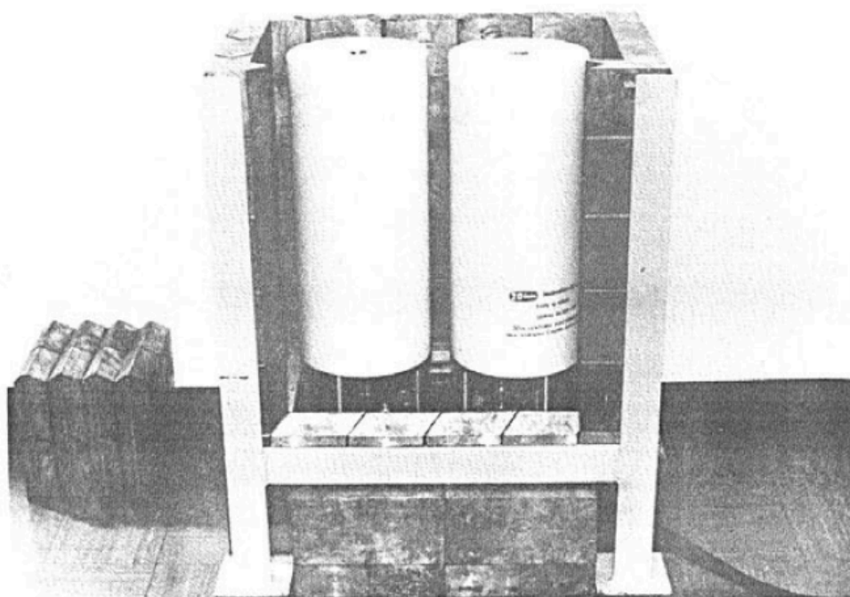
Figure 37-1 — Photograph of the ionization chambers of the SIR (BIPM) mounted in a common lead shield (cover and front wall removed). Reproduced from [376].
