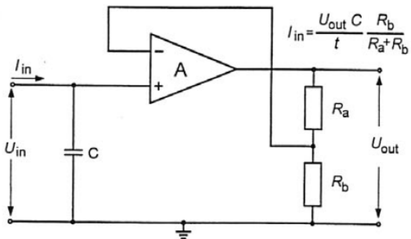
Figure 29-3 — Shunt-type current integrator, with capacitor C and integration time t .
