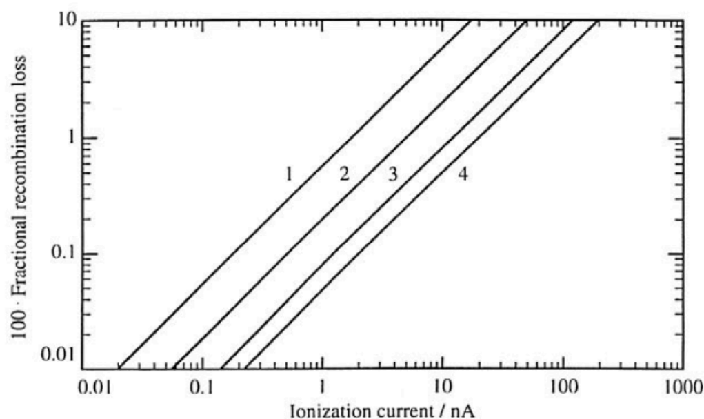
Figure 42 — Recombination loss, expressed as a fraction, in an ionization chamber filled with argon at 1 atm and 23 °C, measured at various collection voltages between the electrodes and plotted versus the ionization current. After Colmenares ([76], see p. 169).
