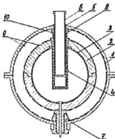
Figure 20 — Spherical 4\pi\gamma -ionization chamber constructed from plastic materials (1, 2) coated with graphite varnish and permitting the introduction of lead or aluminium filters (3). The source is positioned inside a thin metal tube (4). Reproduced from [53].
