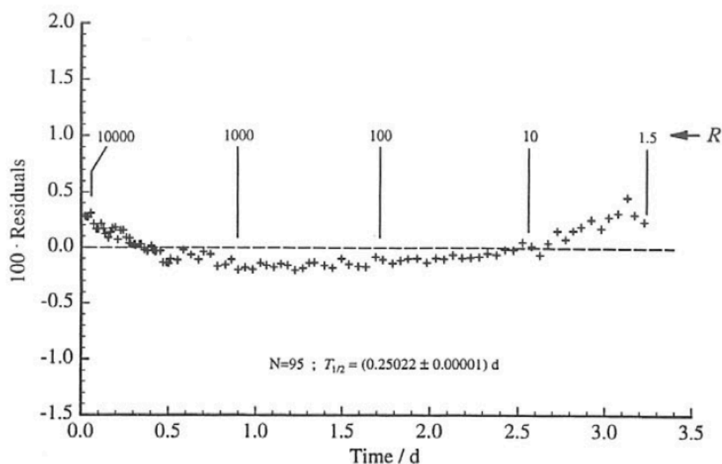
Figure 48-1 — For the full time range of the measurements of longer than twelve times the ^{99}\text{Tc}^{\text{m}} half-life. The residuals show small deviations from linearity at high activity values in the order of a few per mil due to electronic effects and an increasing contribution from ^{99}\text{Mo} at low activity.
