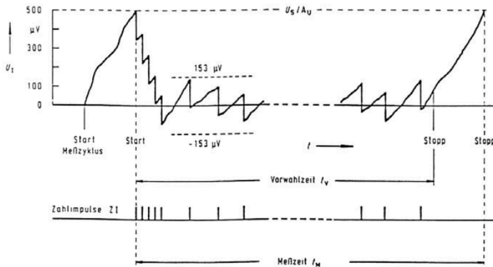
Figure 38-2 — Timing diagram U_I(t) of the PTB induction balance showing a measuring cycle in three parts: The integrated ramp before start up to a voltage level of U_S/A_U , the compensation period between start and stop during which the voltage-frequency converter pulses are counted and the stop ramp to obtain the same voltage level as at start (Meßzyklus \Rightarrow measuring cycle, Vorwahlzeit \Rightarrow preselected time, Zählimpulse \Rightarrow counter pulses, Meßzeit \Rightarrow measuring time, Start \Rightarrow start, Stopp \Rightarrow stop). Reproduced from [104].
