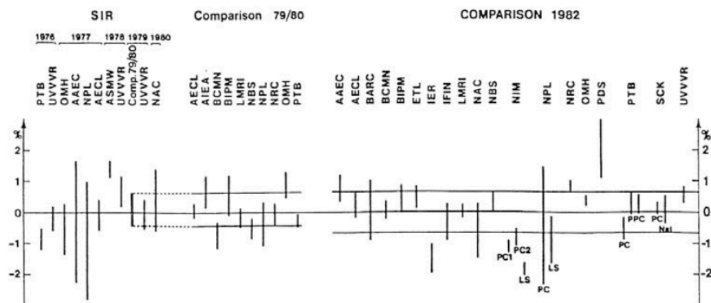
Figure 74 — Graphical representation of the results and their combined uncertainties from comparisons of activity-concentration measurements with ^{137}\text{Cs} . The type of detector is indicated if a laboratory has submitted several results. The mean values of the two comparisons are aligned by means of the corresponding ionization chamber results from the SIR. Their respective standard deviations are represented by pairs of horizontal lines. Reproduced from [377].
