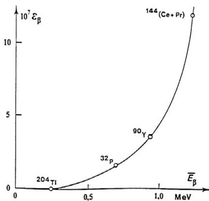
Figure 56-2 — For the ionization chamber of the SIR (BIPM). Reproduced from [384].
