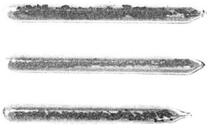
Figure 9 — Three ^{226}\text{Ra} standards prepared by Hönigschmid in 1934, from top to bottom no. 5437 (NIST), no. 5440 (NIST) and no. 5426 (PTB), in the chemical form of radium chloride sealed in glass vials. Reproduced from [295].
