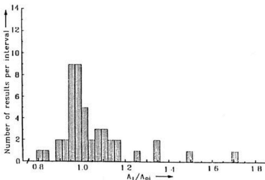
Figure 69-3 — Interval distribution for a ^{123}\text{I} solution in glass vials.
