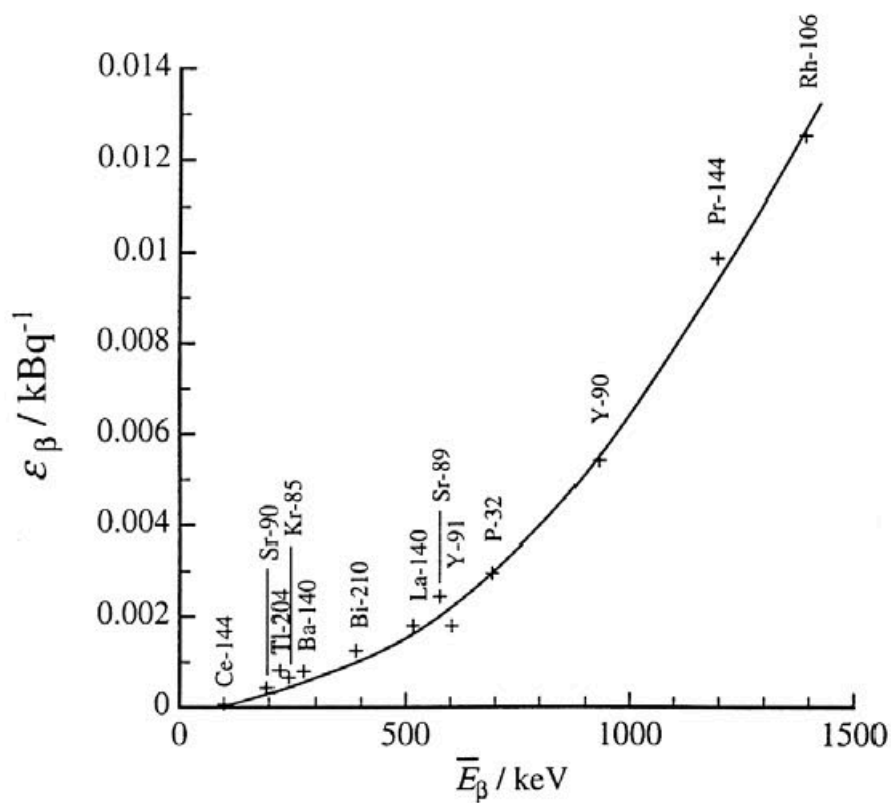
Figure 56-1 — For an ionization chamber, type IG 12 of Centronic, see drawing in Figure 14. (Unpublished data from PTB).
