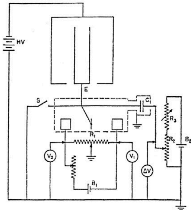
Figure 35-1 — Circuit diagram illustrating the Townsend balance-of-charge system, with semi-automatic compensation: The zero switch is S open, the charge at E is collected and connected to a Lindemann-Ryerson electrometer with quadrant voltages V_1 and V_2 which are adjusted by means of R_1 in the electrical-zero position of the quartz fiber and which corresponds to the mechanical-zero position. The point at E is also connected to the charge-collecting capacitor C and a compensation voltage \Delta V is given on its other side from potentiometer R_2 with battery B_2 , driven by an operator. Reproduced from [164].
