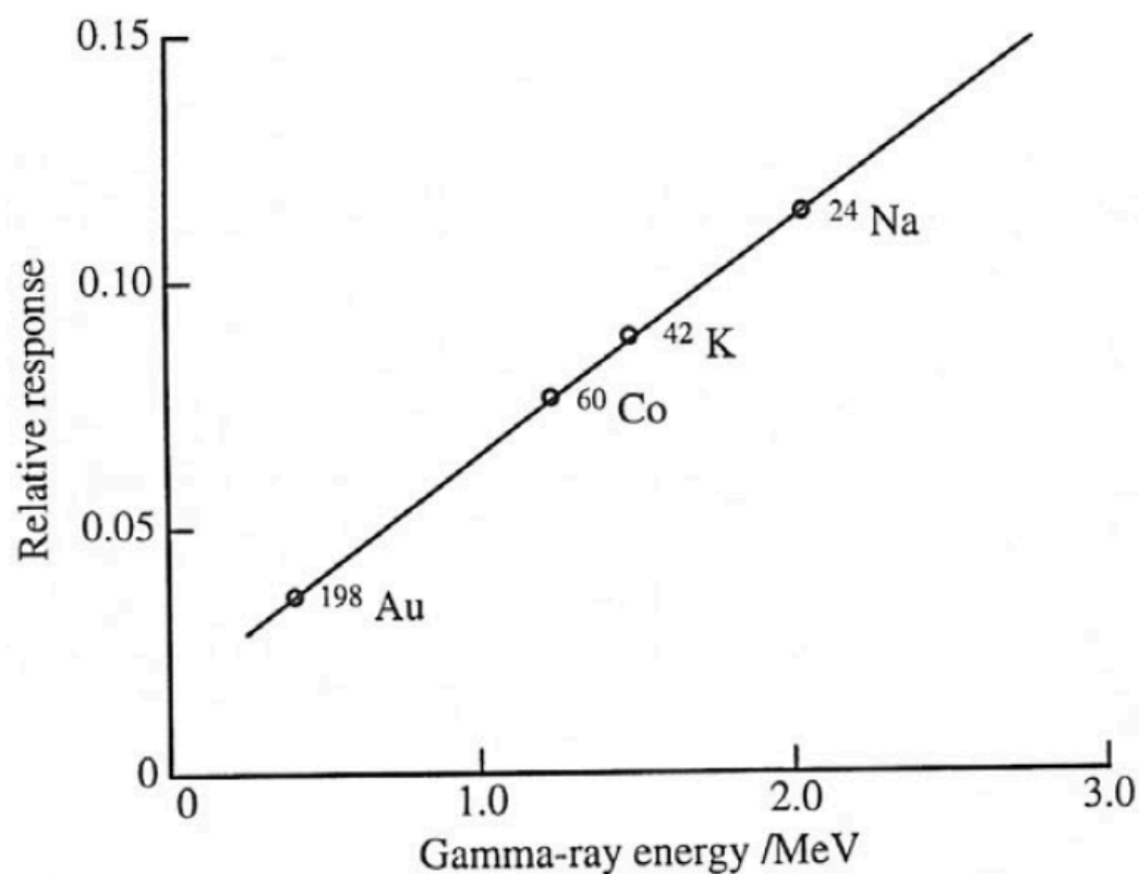
Figure 60-2 — Energy response of the NBS 4πγ-ionization chamber. The current per unit activity has been plotted as a function of the γ-ray energy. Where two γ rays appear in cascade, the energy values have been averaged. It should be possible, knowing the decay scheme of a particular radionuclide, to interpolate and to standardize the disintegration rate of a sample of the nuclide by measurement of the current only. Early data after Mann and Seliger ([295], see p. 183).
