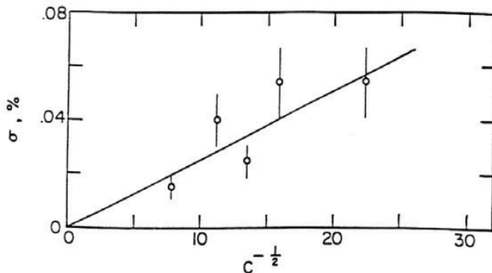
Figure 41-3 — Observed relative standard deviation \sigma as a function C^{-1/2} , where C is the total charge collected per ionization current measurement. Reproduced from [307].
