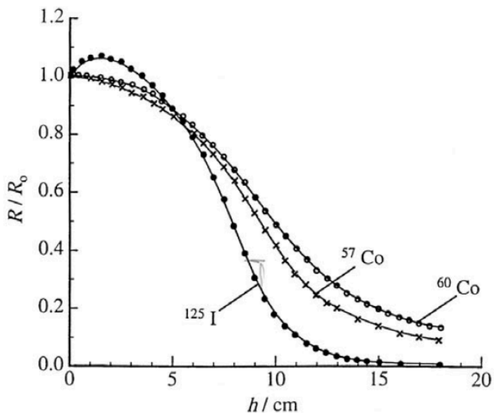
Figure 52-2 — Variation of a radionuclide-calibrator reading R/R_0 , normalized to that of the standard operating position for ^{60}\text{Co} , ^{57}\text{Co} and ^{125}\text{I} . The low-photon energy emitting source of ^{125}\text{I} shows a negative characteristic. Vertical displacement in the well. After Schrader ([398], see p. 190).
