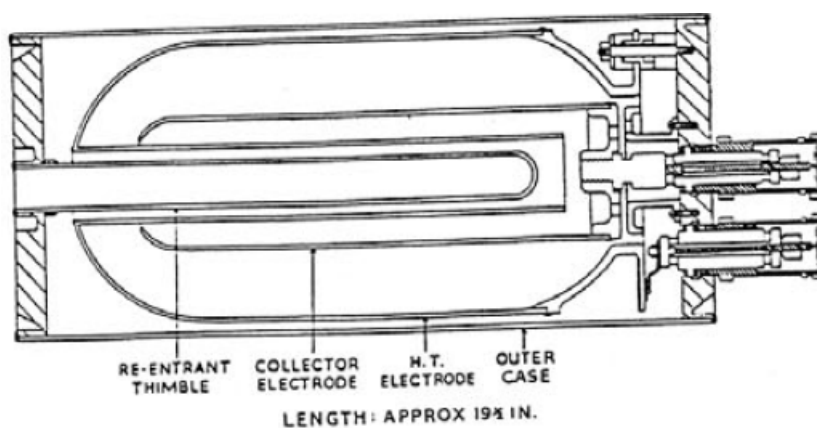
Figure 13 — General arrangement of the redesigned TPA type Mk 2 chamber. The re-entrant thimble for sample insertion and the position of the electrodes can be seen. The chamber is filled with argon of 99.8% purity to a pressure of 20 atmospheres. Reproduced from [406].
