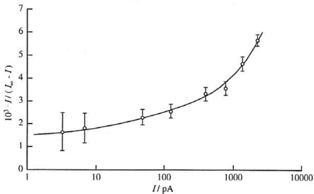
Figure 43-2 — Saturation loss I/(I_\infty - I) as a function of the ionization current I for a chamber at the PTB. After Weiss ([469], see p. 194).
