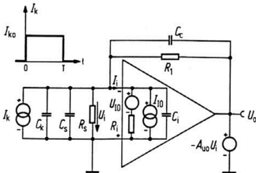
Figure 30 — Current-integrator equivalent-circuit diagram to study the parameters of a measuring system, such as leakage currents or the time dependence of integration for a current pulse of duration T (on top left), with the current to be measured I_k , input current I_i , initial-offset current I_{10} , input voltage U_i , initial-offset voltage U_{10} , output voltage U_o , open-loop gain A_{u0} , input resistance R_i , feedback resistance R_1 , stray resistance R_s , stray capacity C_s , capacity of the current source C_k , input capacity C_i and feedback capacity C_c . Reproduced from [34] and [37].
