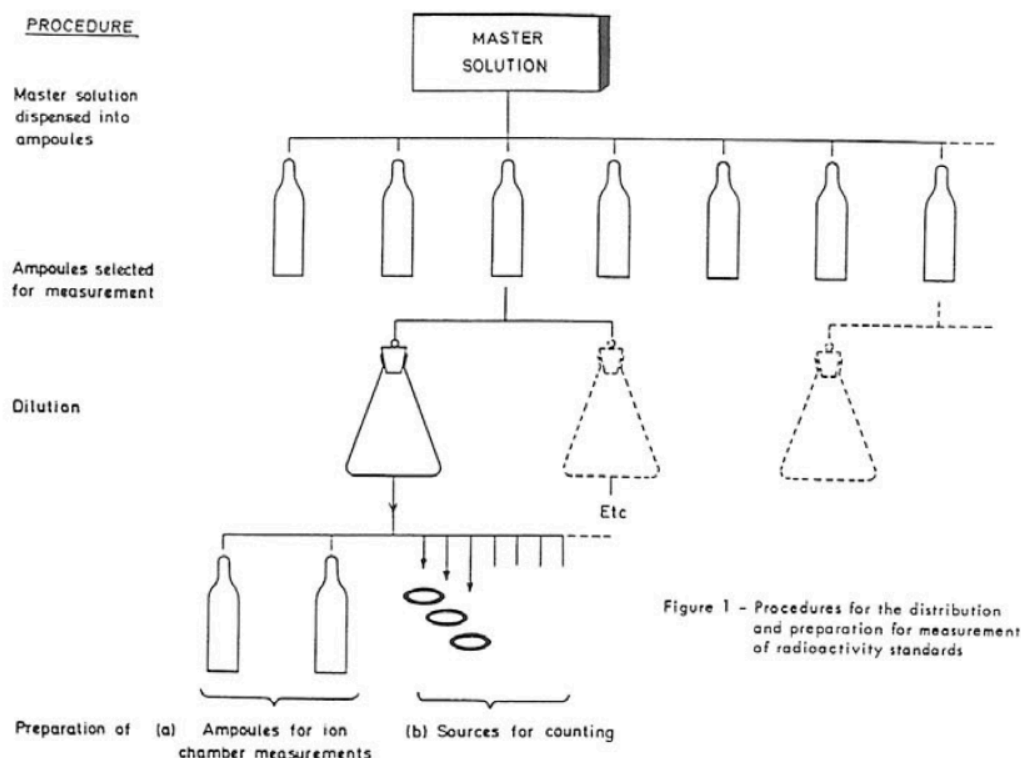
Figure 68-1 — Procedures for the distribution and preparation for measurement of radioactivity standards. The dilution steps are shown in a family of solutions dispensed into ampoules or dripped on foils for solid sources. Each step is followed by weighing procedures and controlled by measurements. Reproduced from the monograph of Campion, BIPM ([63], see p. 168).
