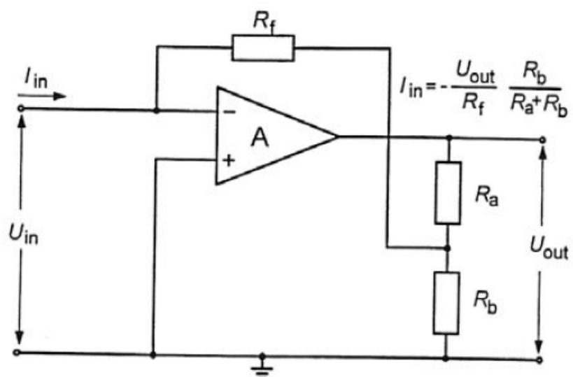
Figure 29-2 — Feedback-type picoamperemeter, with feedback resistor R_f .
