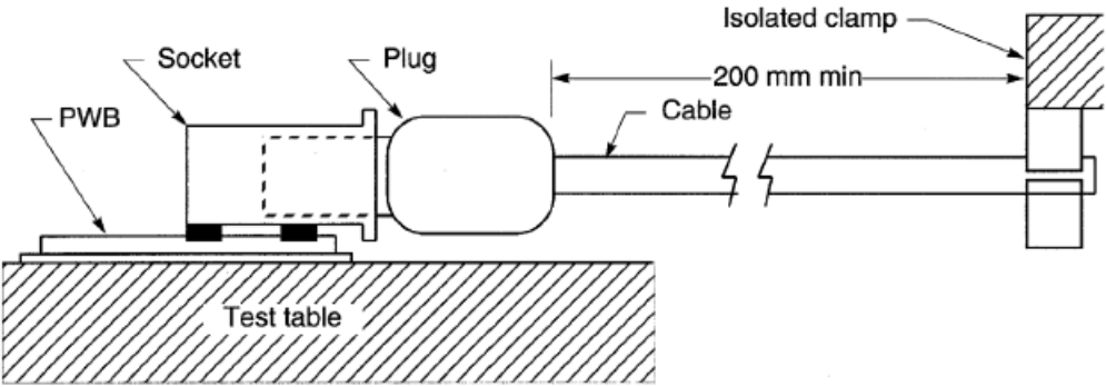
1 Figure 2-1—vibration test
