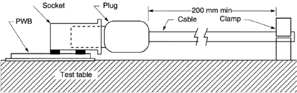
2 Figure 2-2—shock test
