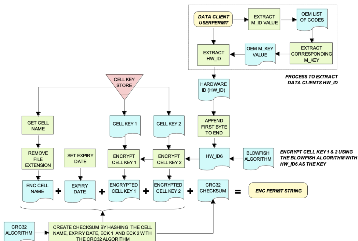
Figure 10-6 — Data Server Process - Create Cell Permit
