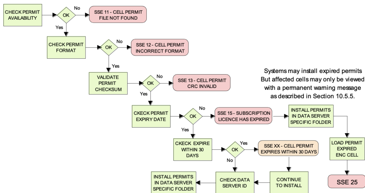
Figure 11-3 — OEM System - Install & Validate Cell Permit
