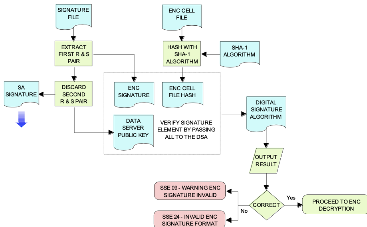
Figure 11-5 — Authenticate ENC Cell File - Validate ENC Signature
