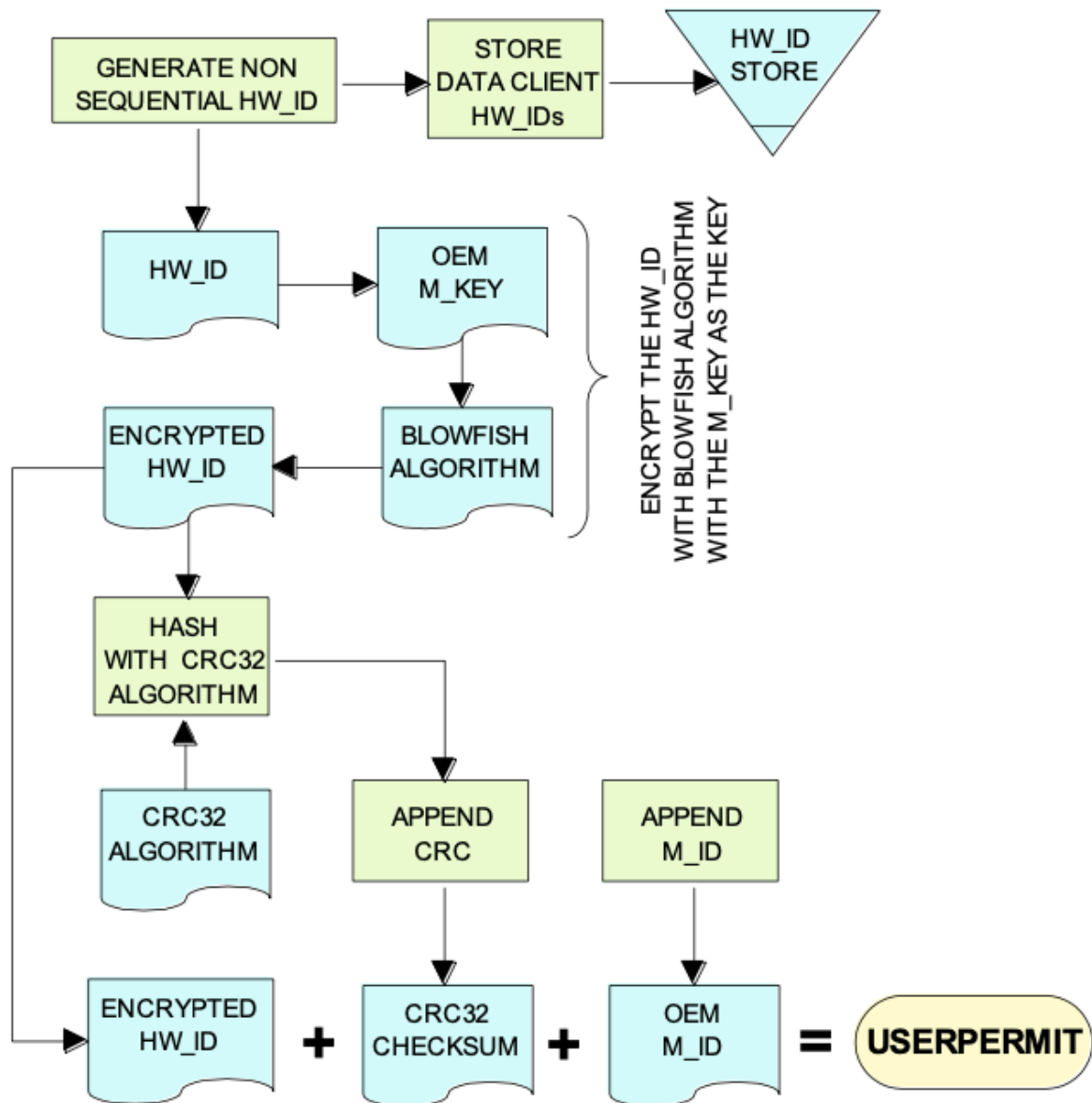
Figure 11-2 — OEM - Create Userpermit
