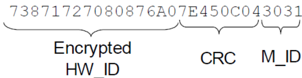
Userpermit Structure
