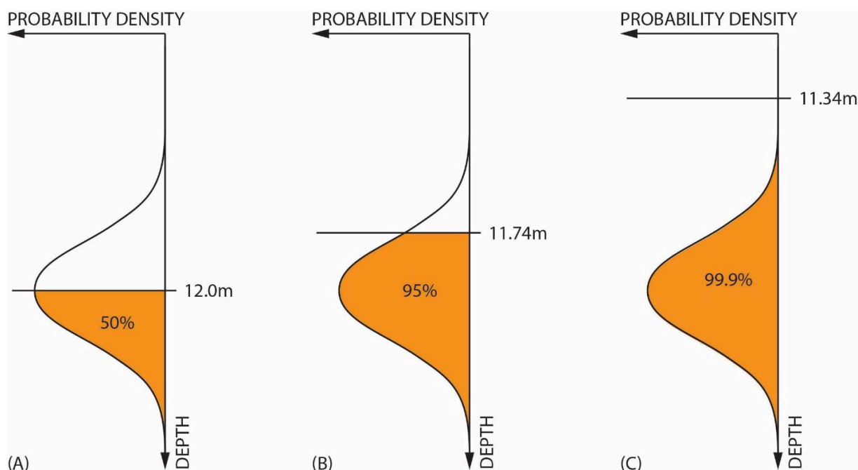
Figure 4-7 — Examples of shoal-clearance depths for different probabilities of excursion, based on the same basic uncertainty estimate of 12.0 \pm 0.3 m (95% CI). Assuming a 12.0m clearance is only true 50% of the time (left); a 5% probability of being shallower requires the depth to be reduced to 11.74m (middle); a 1:1000 chance of being shallower requires a clearance depth of 11.34m (right).
