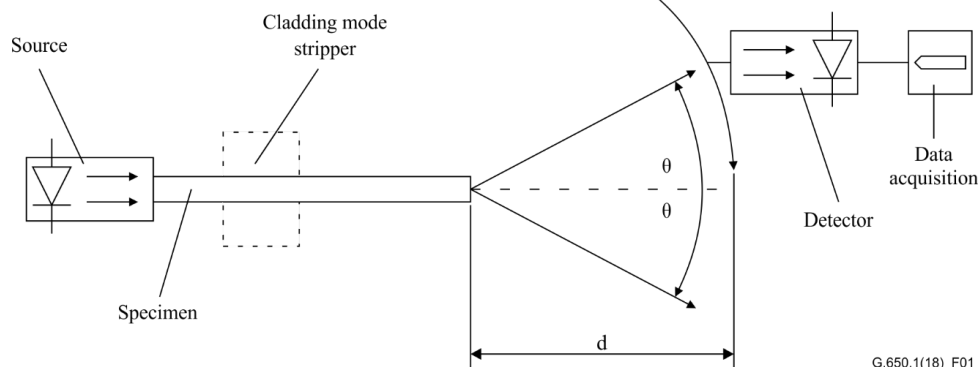
Figure 1 — Typical arrangement of the far-field scan set-up
