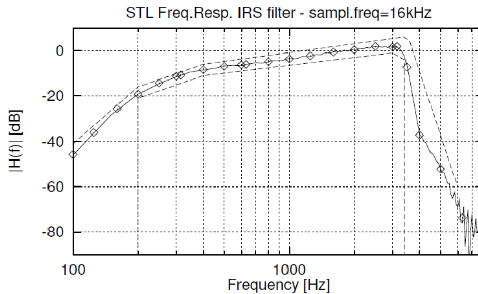
Figure 31-b — Transmission-side IRS for input samples at 16 kHz
