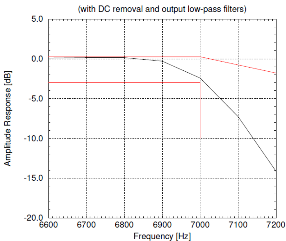
Figure 86-b — Wideband Duo-MNRU
