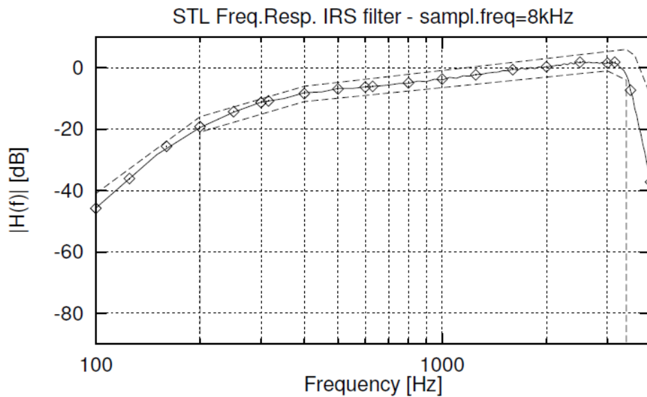
Figure 31-a — Transmission-side IRS for input samples at 8 kHz
