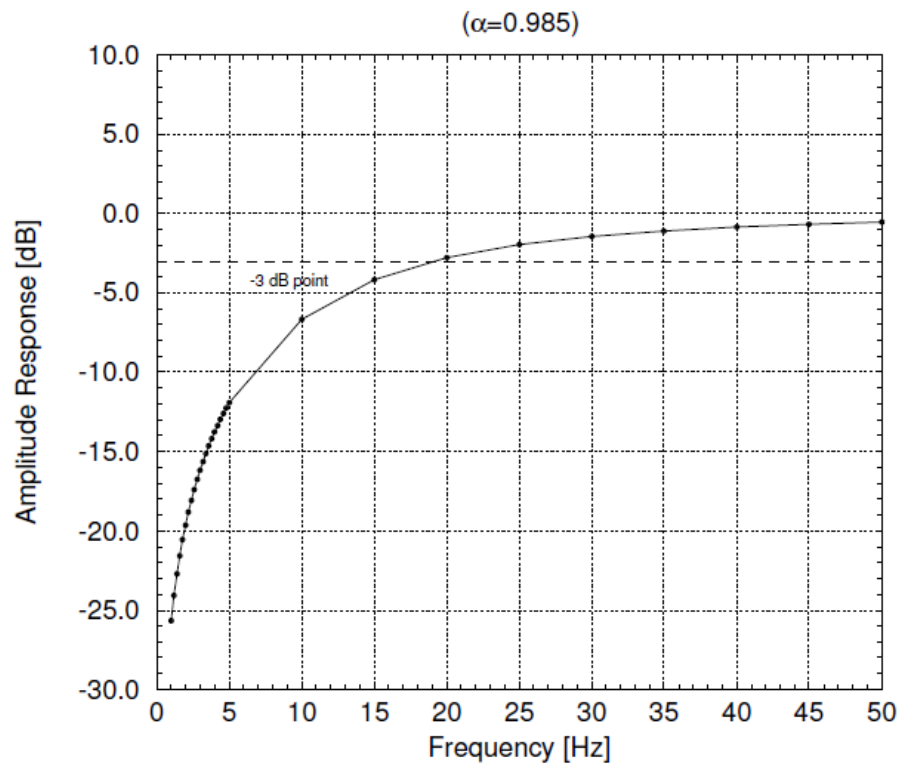
Figure 85-a — Narrowband Duo-MNRU
