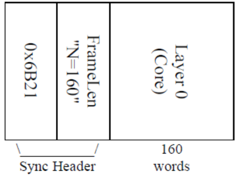
Figure 76 — Example G.192 output frame when layer 1, layer 3 and layer 4 are hit by layer errors in the layered error application mode
