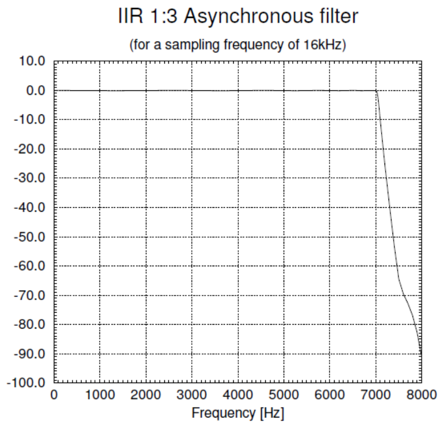
Figure 65-a — Flat low-pass up-sampling by a factor of 1:3
