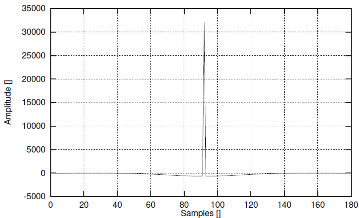
Figure 30 — STL MSIN send-side filter impulse response
