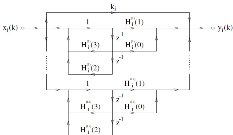
Figure 87 — MNRU Filters Structure
