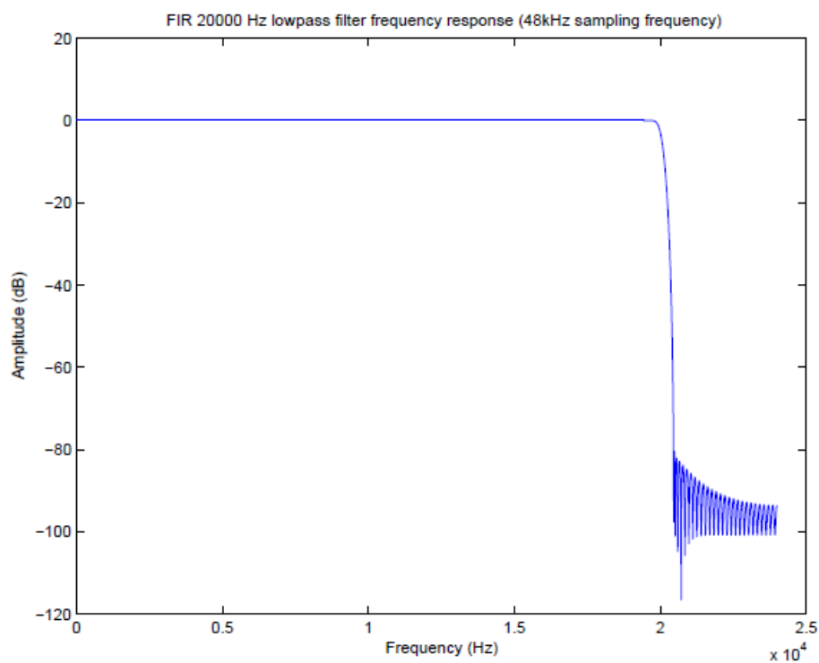
Figure 61 — Frequency response of the STL MUSHRA anchor LP20—Low-pass filter with cut-off frequency 20 kHz for a sampling frequency of 48 kHz (factor 1:1)
