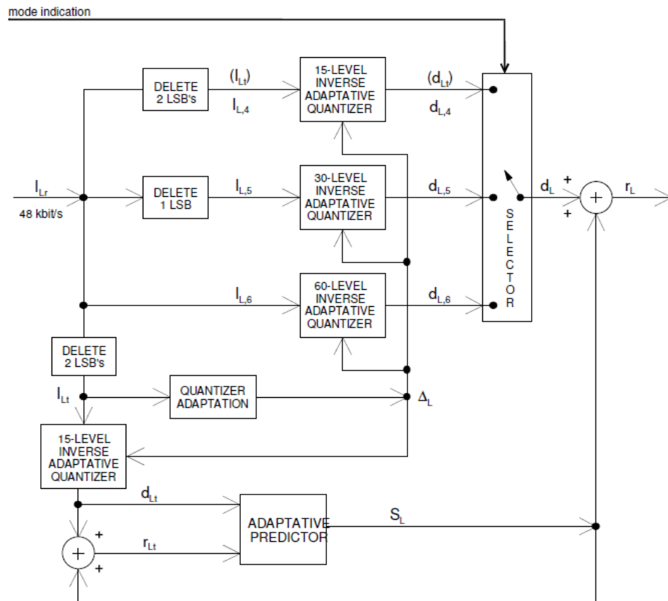
Figure 12 — Block diagram of the SB-ADPCM decoder
