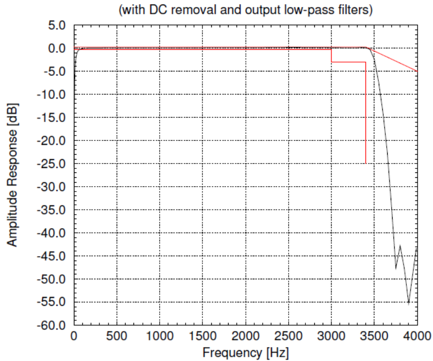
Figure 84-a — Narrowband Duo-MNRU
