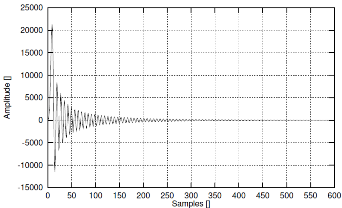
Figure 66-a — 1:3 up-sampling factor
