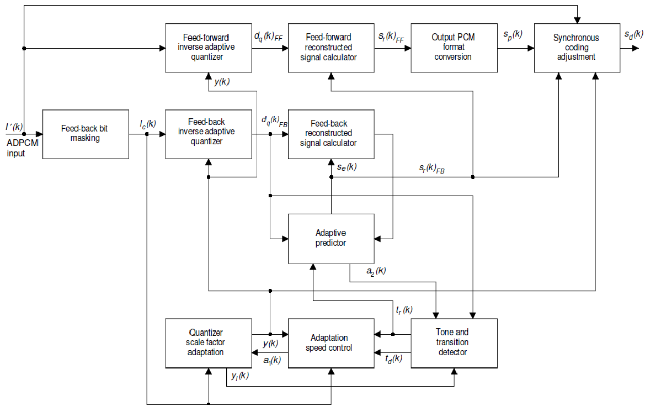
Figure 4-b — Decoder
