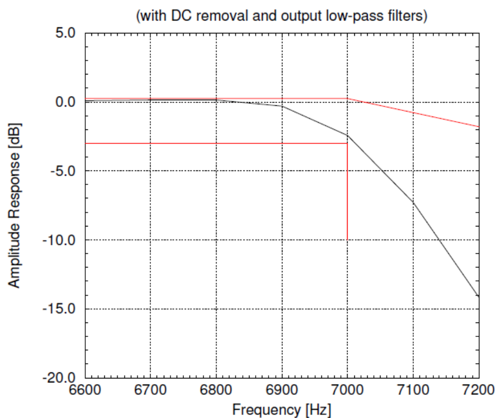
Figure 86-b — Wideband Duo-MNRU
