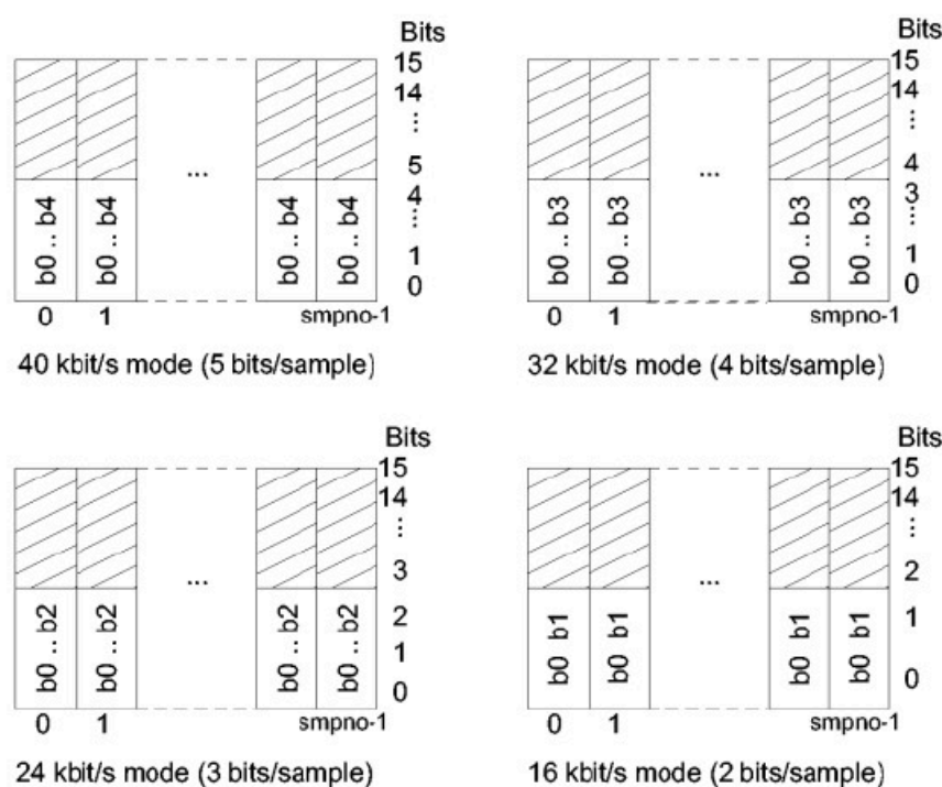
Figure 3 — Packing of G.726-encoded signals (right-aligned, parallel format)
