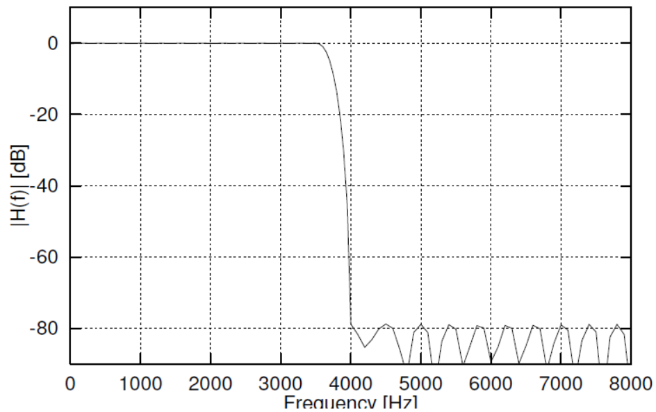
Figure 23-b — High-quality filter for down-sampling
