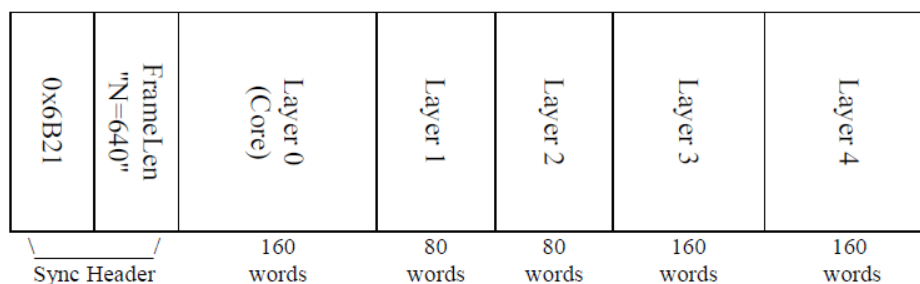
Figure 73 — Example G.192 input frame with layering "-layers 160,240,320,480,640". This frame has a size of 640 bits and a G192 SYNC(0x6B21) header tag
