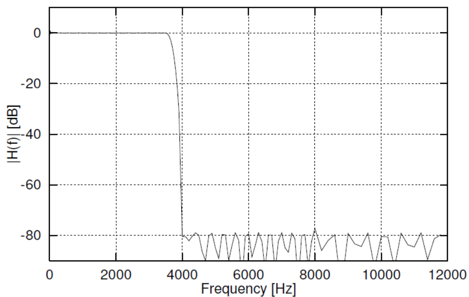
Figure 24-b — High-quality filter for down-sampling
