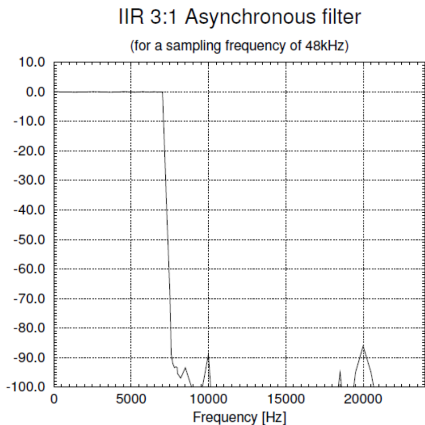
Figure 65-b — Flat low-pass down-sampling by a factor of 3:1
