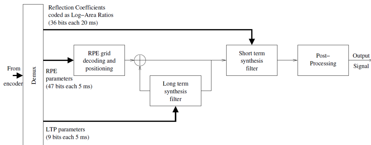
Figure 19 — Simplified block diagram of the RPE-LTP decoder
