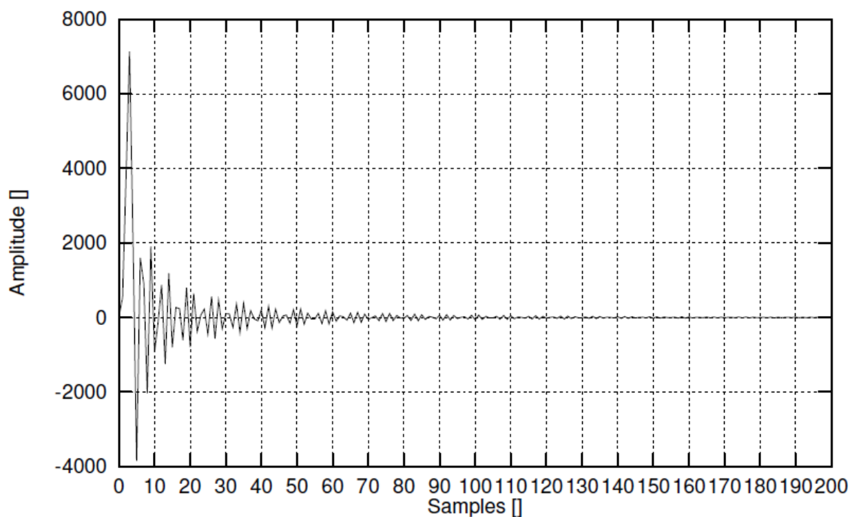
Figure 66-b — 3:1 down-sampling factor
