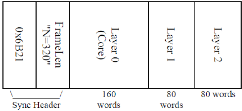
Figure 75 — Example G.192 output frame when layer 3 is hit by a layer error in the layered error application mode
