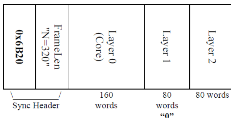
Figure 79 — Example G.192 output frame when layers 1, 3 and 4 are hit by layer errors in the individual error application mode. Note that the frame is truncated and that the Sync header is changed to G192 FER(0x6B20) to indicate the presence of layers with remaining errors
