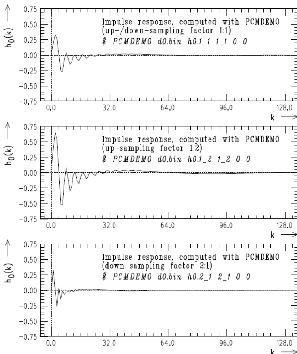
Figure 68 — Impulse response for G.712 filters (Top: factor 1:1; Middle: factor 1:2; Bottom: factor 2:1)
