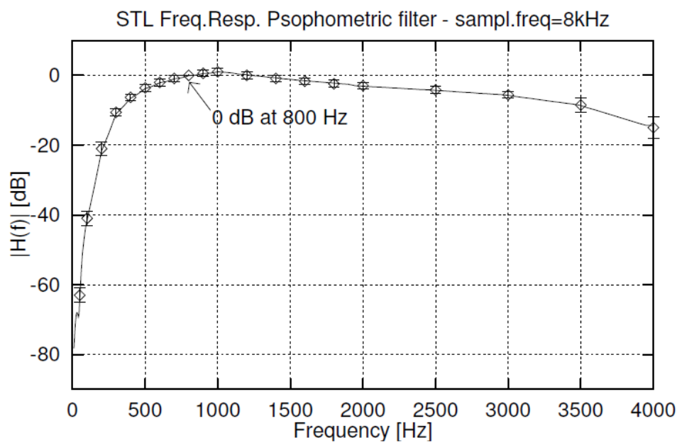
Figure 37 — Frequency response for the psophometric filter. The points show the average points and the allowed range as per ITU-T Rec. O.41
