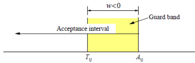
Figure 11 — Decision rule based on guarded rejection. An upper acceptance limit A_U outside an upper tolerance limit T_U defines an acceptance interval that reduces the probability of falsely rejecting a conforming item (producer's risk). The length parameter w associated with a guarded rejection guard band is w = T_U - A_U < 0 .
