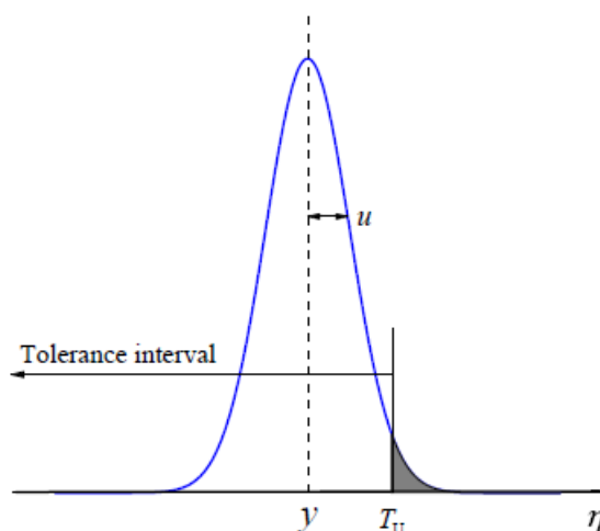
Figure 4 — As Figure 3 except with a single upper tolerance limit T_U . Conforming values of Y lie in the interval \eta \leq T_U .
