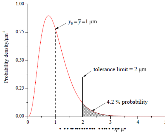
Figure 14 — Gamma prior PDF given by Equation (23), assigned based on the frequency distribution of measured radial error motions for a sample of ball bearings. The tolerance interval is the region 0 \leq \eta \leq 2 \mu\text{m} . The expectation of the distribution is the prior estimate y_0 = 1 \mu\text{m} , with an associated standard uncertainty u_0 = 0.5 \mu\text{m} . Because the distribution is not symmetric, the most probable value of Y (the mode of the distribution, here equal to 0.75 \mu\text{m} ) is not equal to y_0 .
