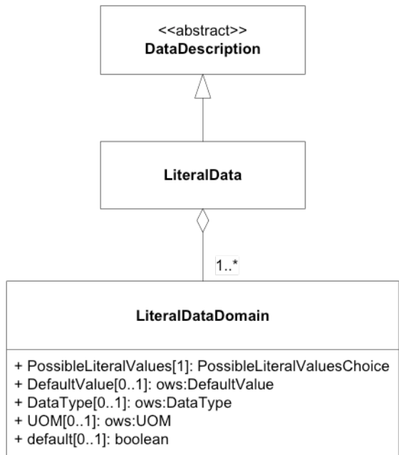
Figure 9 – LiteralData UML class diagram
