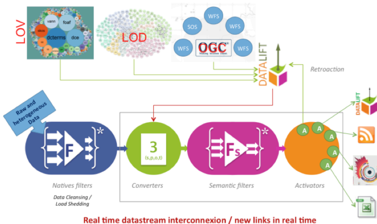
Figure 17 — Creating linked data in real time (Figure Source: G. Kepekian)
