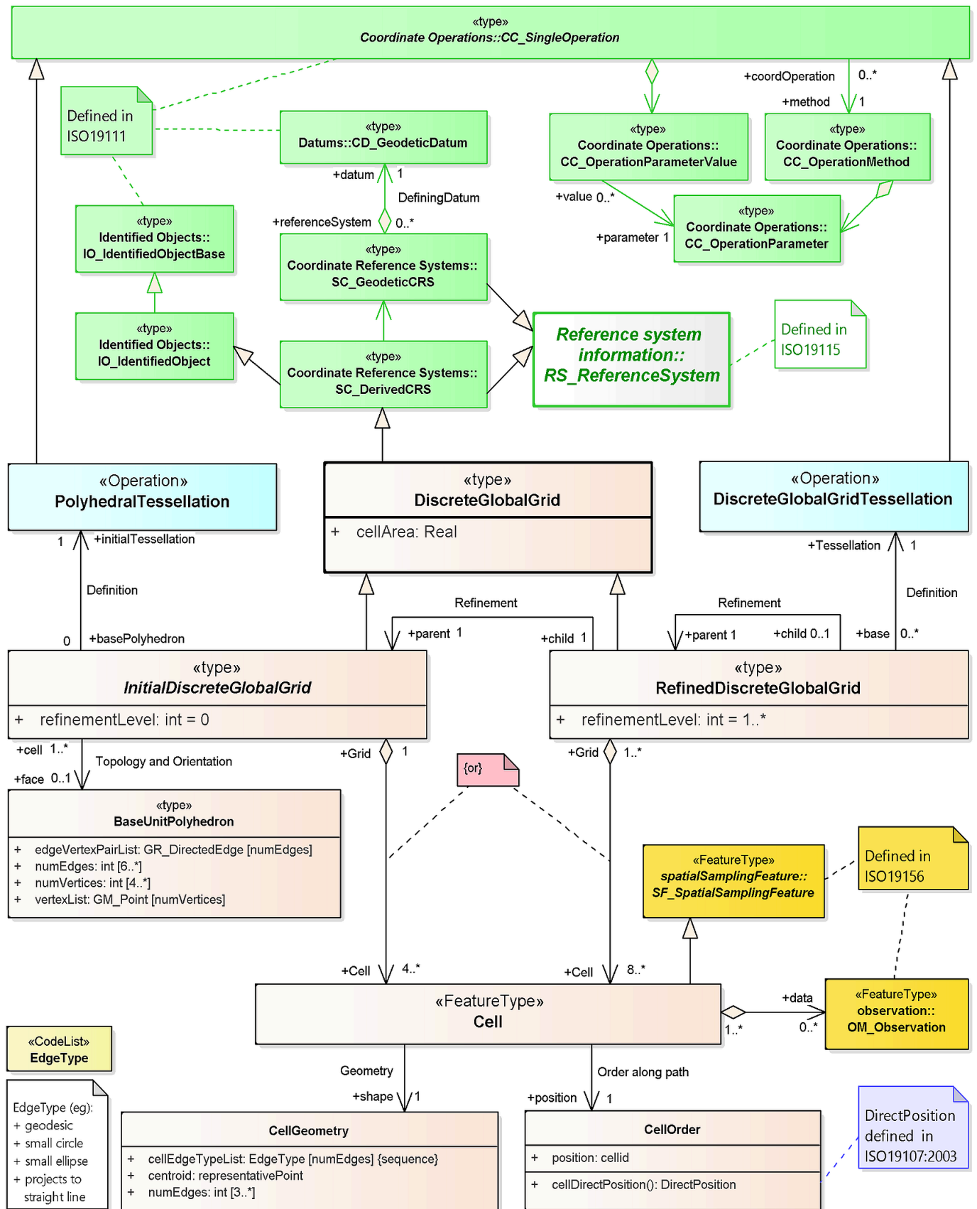
Figure 8 – DGGS Reference Frame Class diagram
