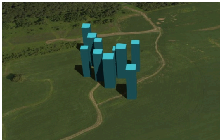
Figure 2 — A parent tile with replacement refinement
