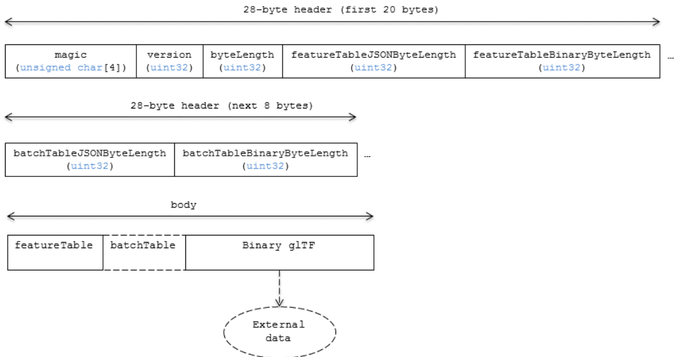
Figure 24 — Batched 3D Model layout
