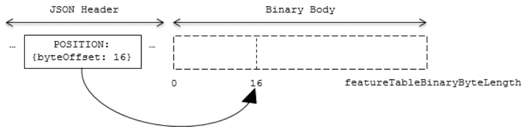
Figure 21 — Feature Table binary body layout
