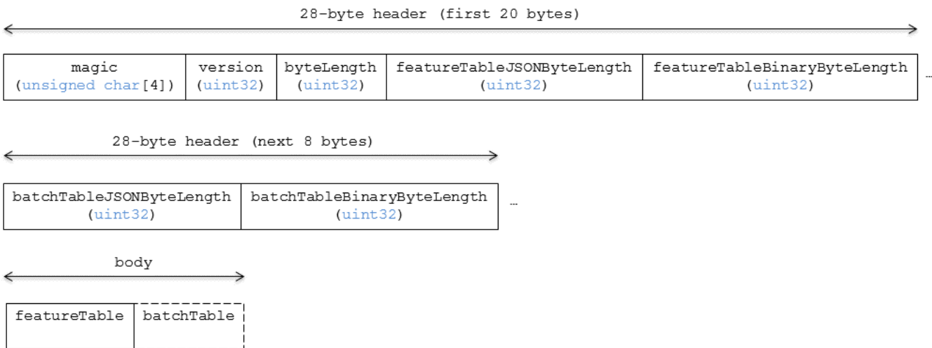
Figure 29 — Point Cloud layout
