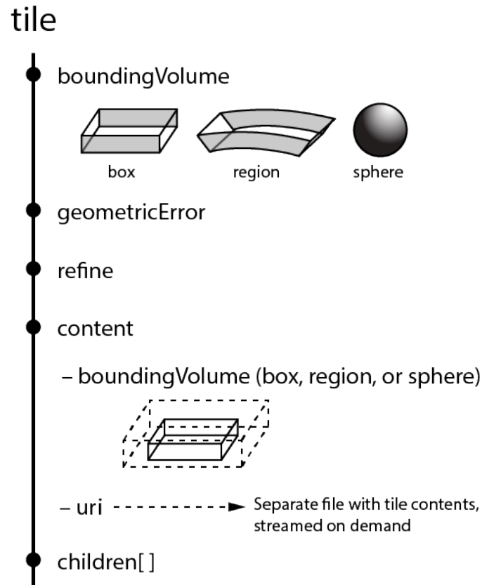
Figure 13 – Tile JSON properties
