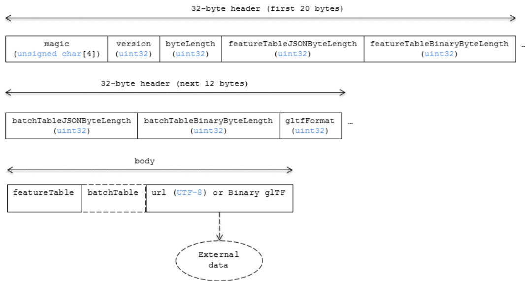
Figure 25 — Instanced 3D Model layout
