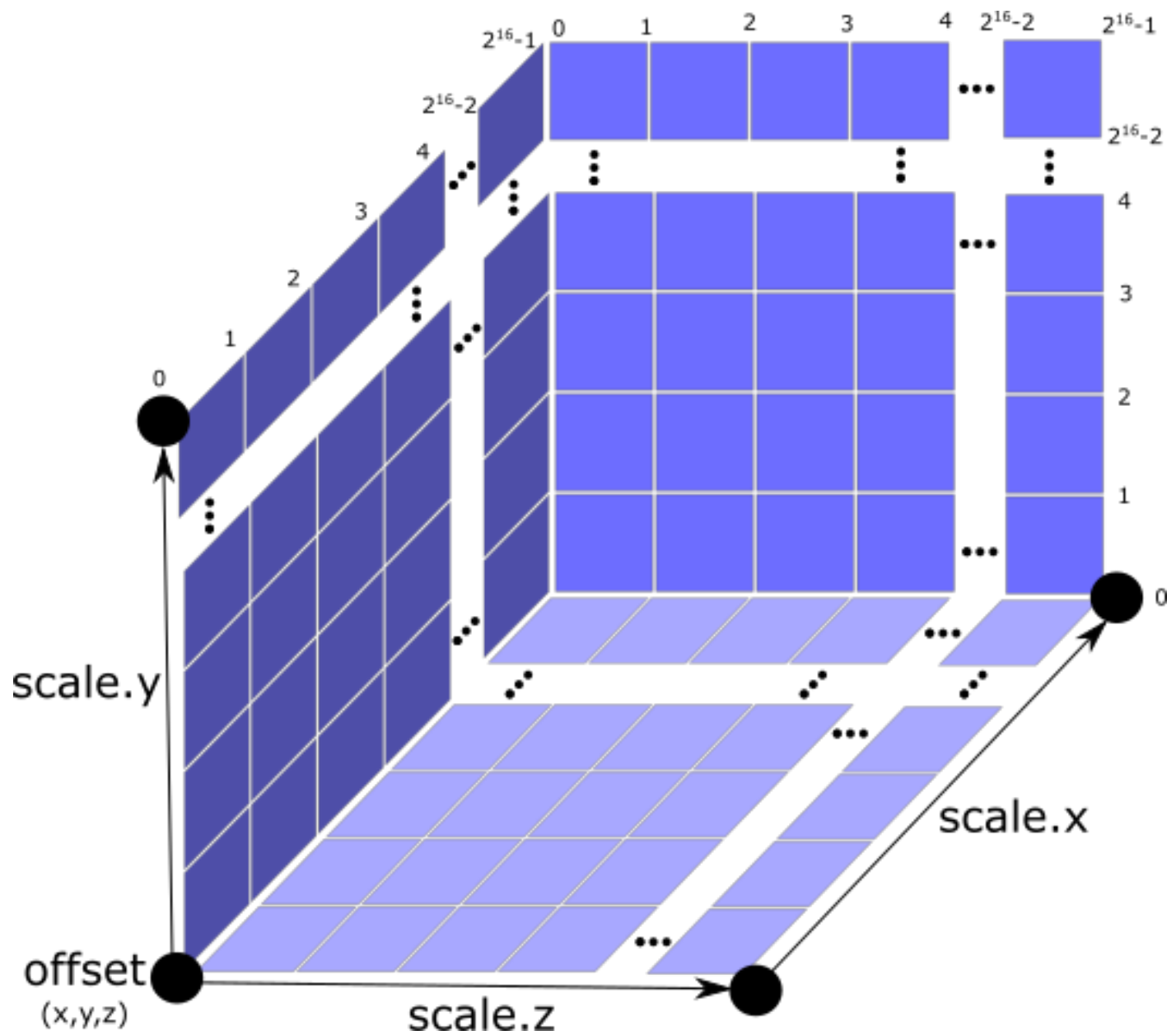
Figure 30 — A quantized volume
