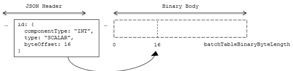
Figure 23 – Batch Table binary body layout
