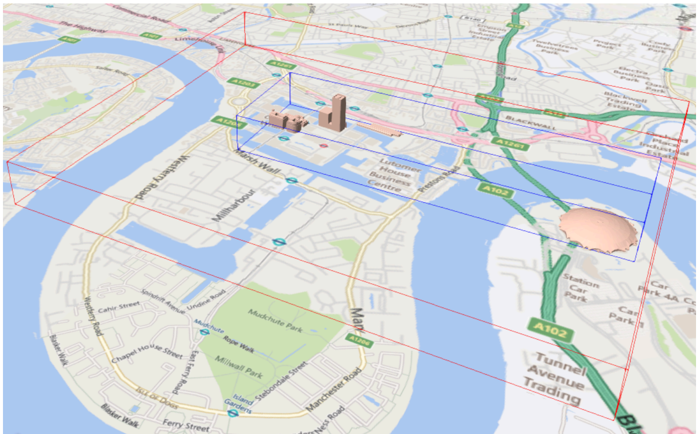
Figure 14 — A tile bounding volume in red, and a content bounding volume in blue
