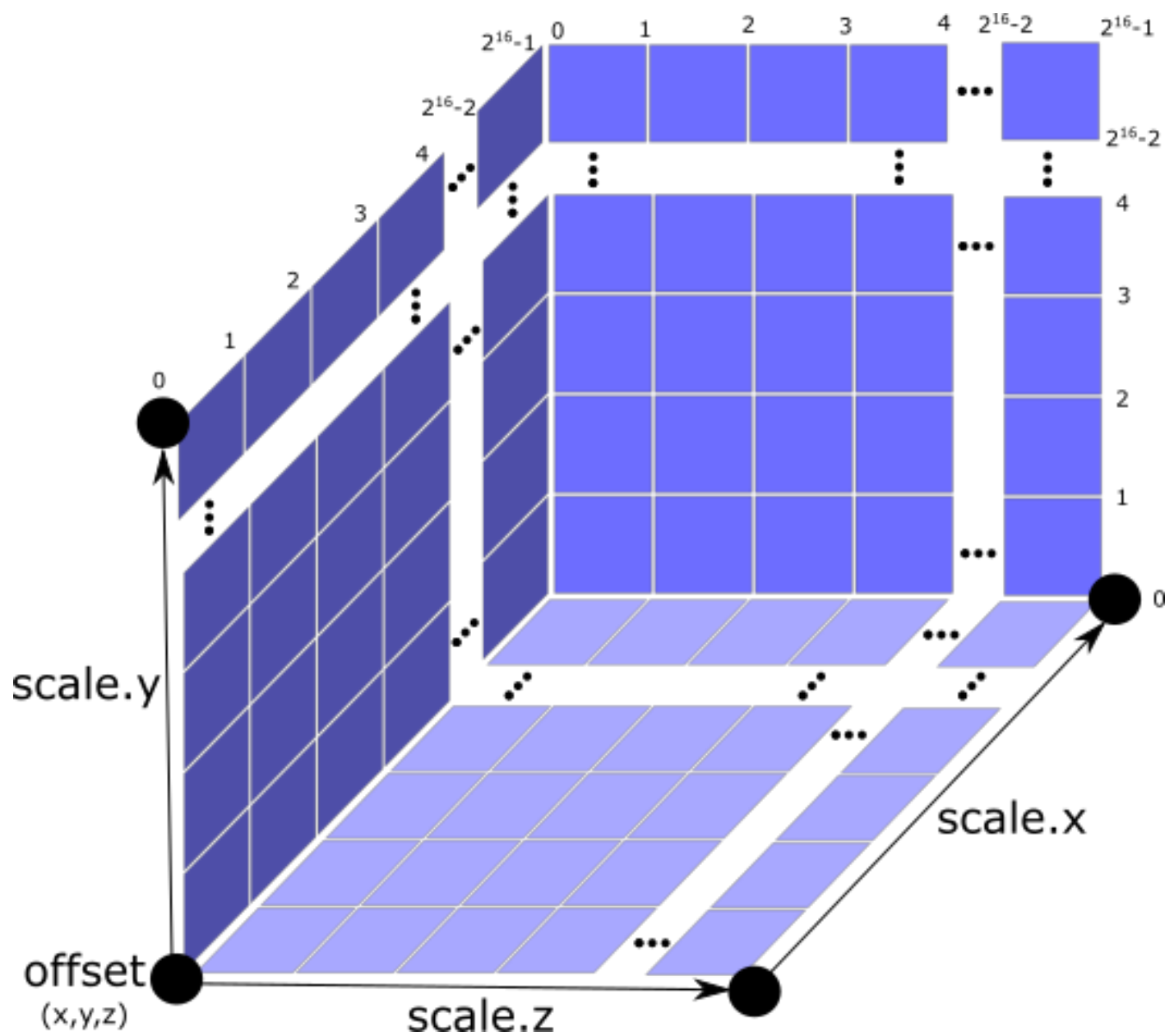
Figure 28 — A quantized volume
