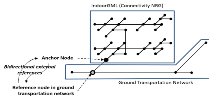
Figure 16: Anchor Node Connecting Indoor and Outdoor Networks [27]
