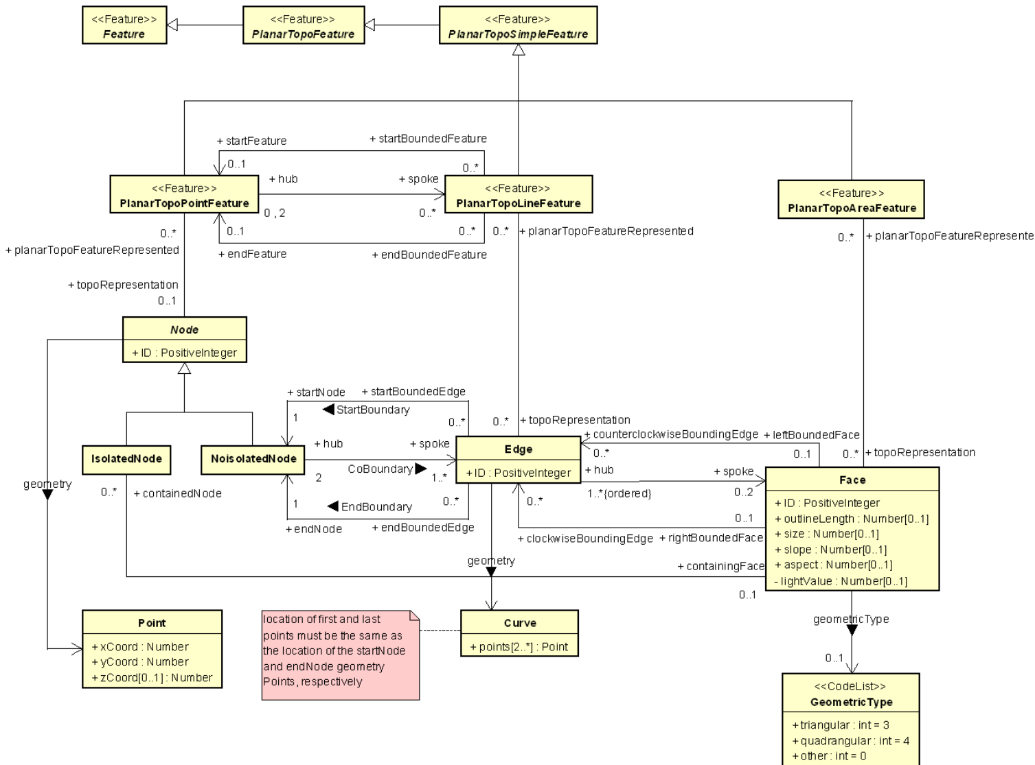
Figure 29 – UML diagram of the conceptual data model for 'PlanarTopoSimpleFeature'
