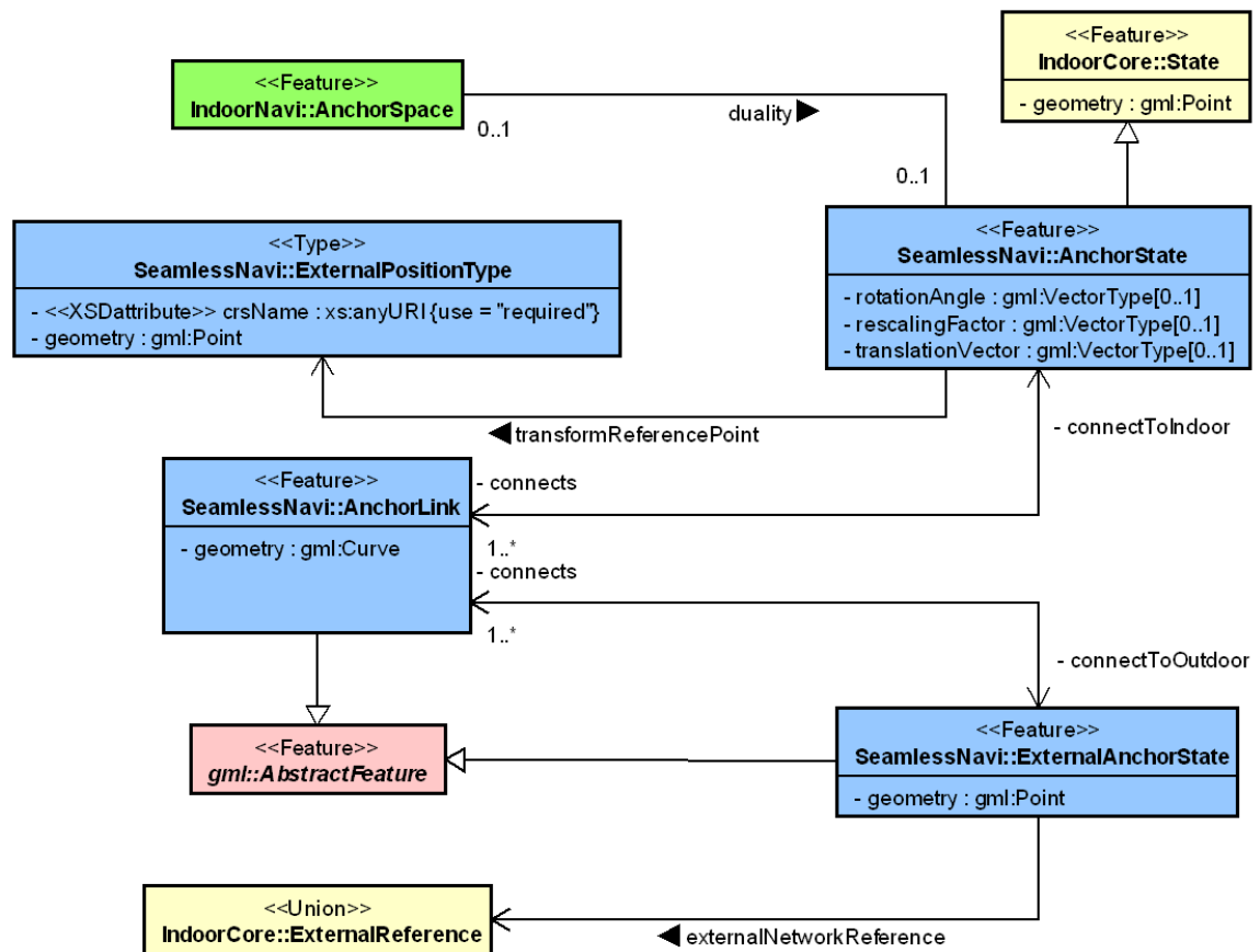
Figure 8 – UML diagram for SeamlessNavigation module (simple version)
