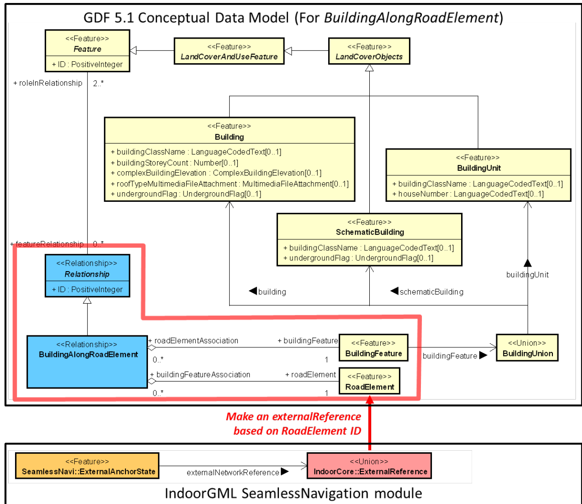
Figure 27 – UML diagram of the conceptual data model for 'Relationships' with 'BuildingAlongRoadElement'
