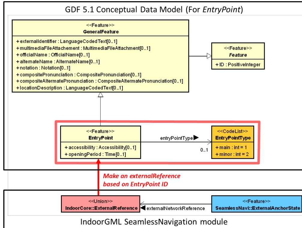
Figure 28 – UML diagram of the conceptual data model for EntryPoint of General Feature
