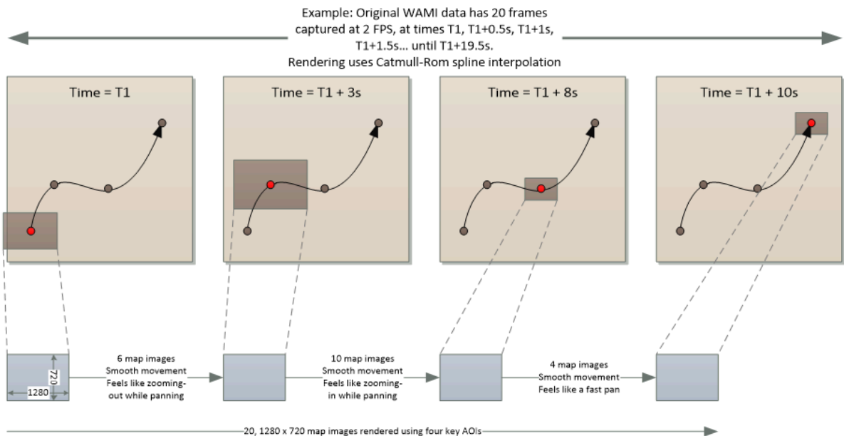
Figure 14 – Key-frame animation using GetPathMap and GetPathMapVideo
